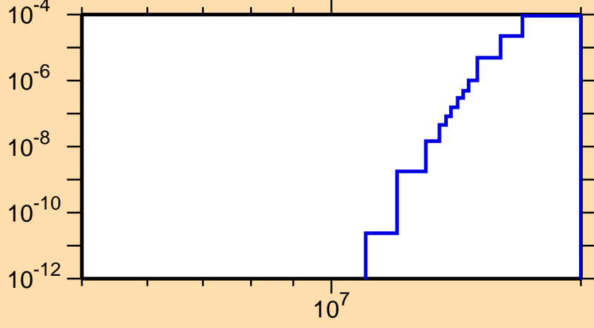
\sigma vs. E for ^{234}\text{Ra}(n,t)
