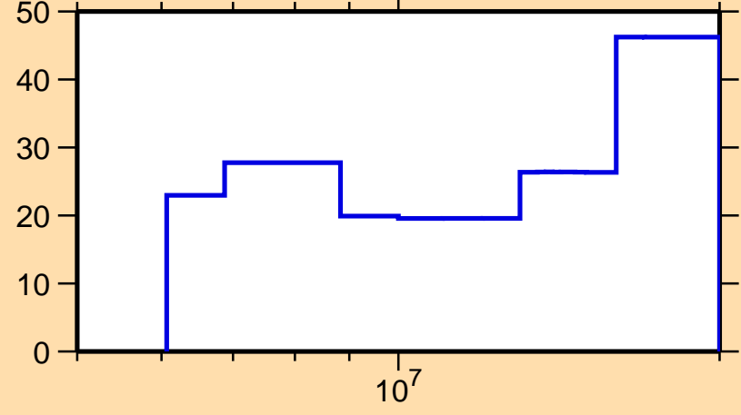
\Delta\sigma/\sigma vs. E for ^{234}\text{Ra}(n,el.)
