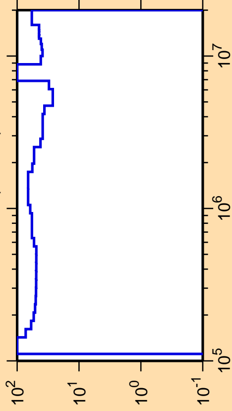
\Delta\sigma/\sigma vs. E for ^{234}\text{Ra}(n,\text{inel.})
