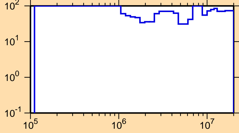
\Delta\sigma/\sigma vs. E for ^{234}\text{Ra}(n,n\text{cont.})
