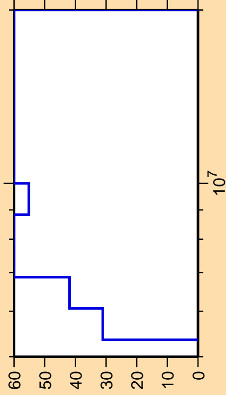
\Delta\sigma/\sigma vs. E for ^{234}\text{Ra}(n,n\text{cont.})
