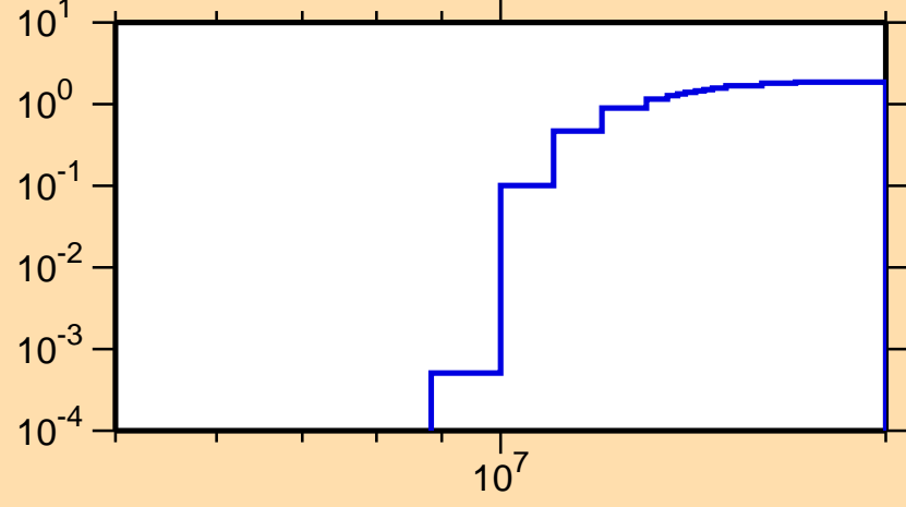
\sigma vs. E for ^{234}\text{Ra}(n,3n)
