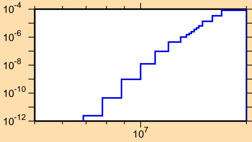
\sigma vs. E for ^{234}\text{Ra}(n,\alpha)
