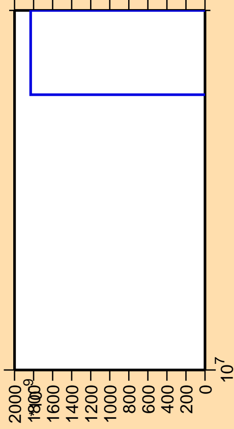
\Delta\sigma/\sigma vs. E for ^{234}\text{Ra} (mt 42)
