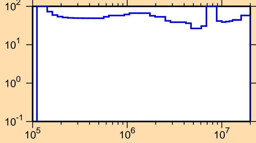
\Delta\sigma/\sigma vs. E for ^{234}\text{Ra}(n,\text{inel.})
