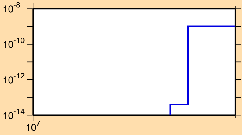
\sigma vs. E for ^{234}\text{Ra}(n,2np)
