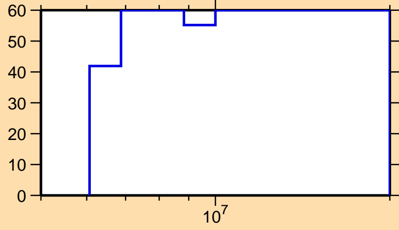
\Delta\sigma/\sigma vs. E for ^{234}\text{Ra}(n,n\text{cont.})
