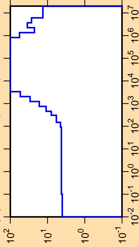
\Delta\mu/\mu vs. E for ^{234}\text{Ra}(\text{mt251})
