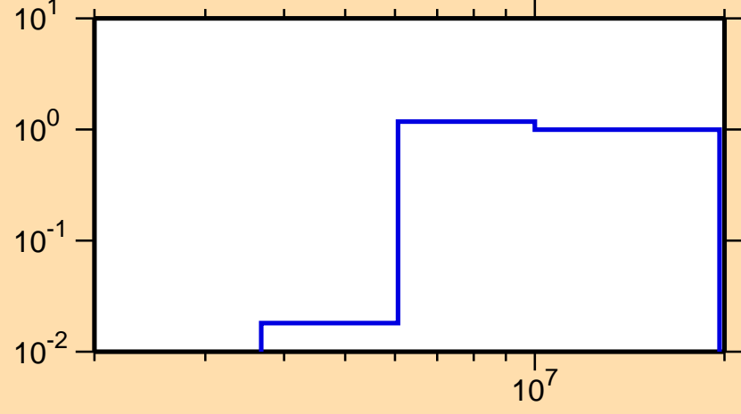
\sigma vs. E for ^{234}\text{Ra}(n,2n)
