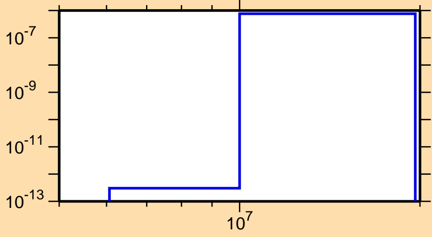
\sigma vs. E for ^{234}\text{Ra}(n,n\alpha)
