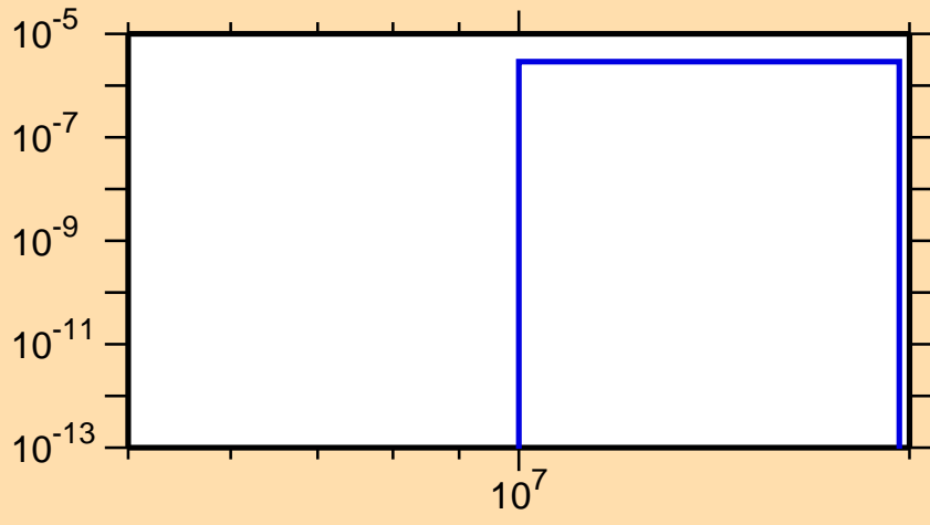
\sigma vs. E for ^{234}\text{Ra}(n,t)
