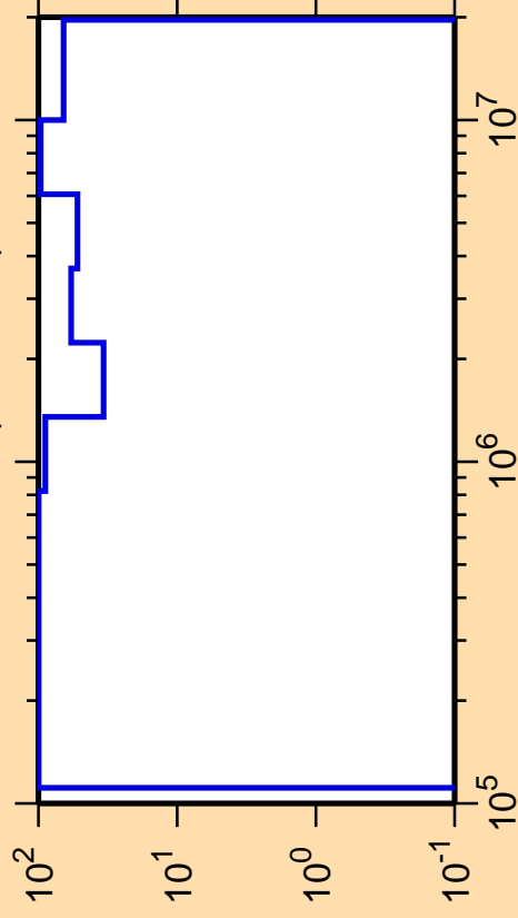
\Delta\sigma/\sigma vs. E for ^{234}\text{Ra}(n,\text{ncont.})
