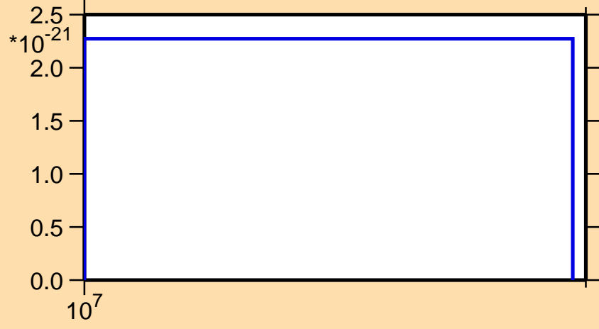
\sigma vs. E for ^{234}\text{Ra} (mt 42)
