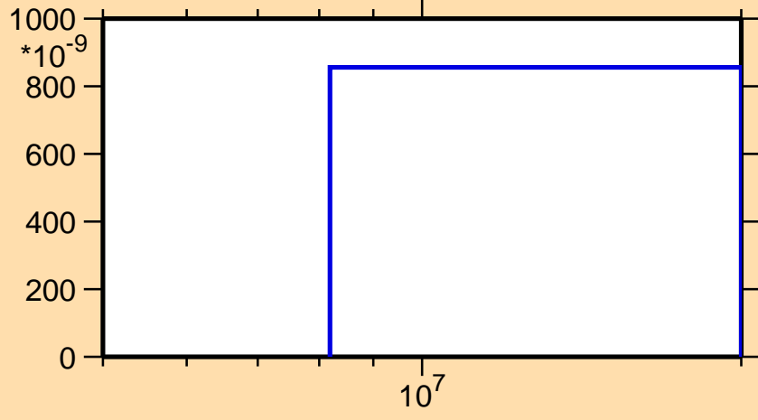
\sigma vs. E for ^{234}\text{Ra}(n,np)
