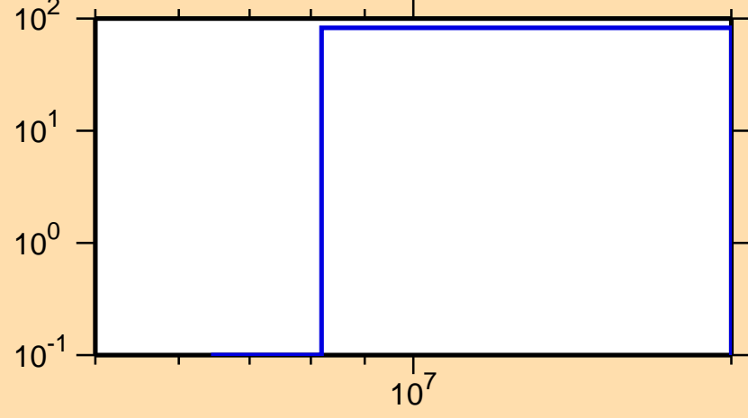
\Delta\sigma/\sigma vs. E for ^{234}\text{Ra}(n,p)
