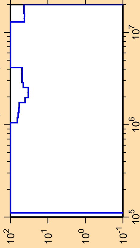
\Delta\sigma/\sigma vs. E for ^{235}\text{Ra}(n,\text{ncont.})
