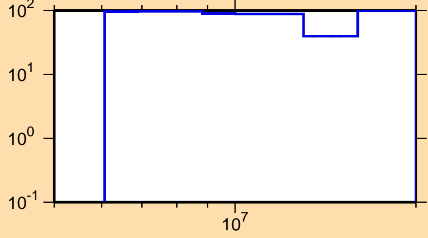
\Delta\sigma/\sigma vs. E for ^{235}\text{Ra}(n,\gamma)
