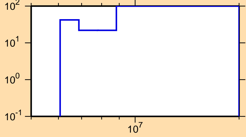
\Delta\sigma/\sigma vs. E for ^{235}\text{Ra}(n,2n)
