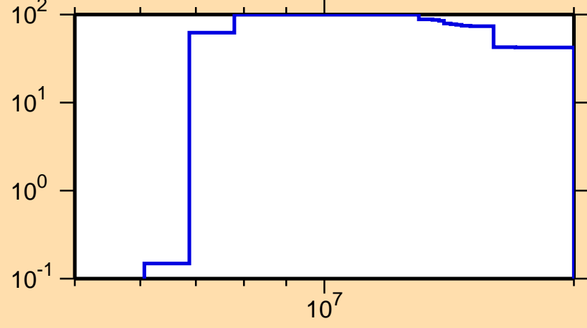
\Delta\sigma/\sigma vs. E for ^{235}\text{Ra}(n,p)
