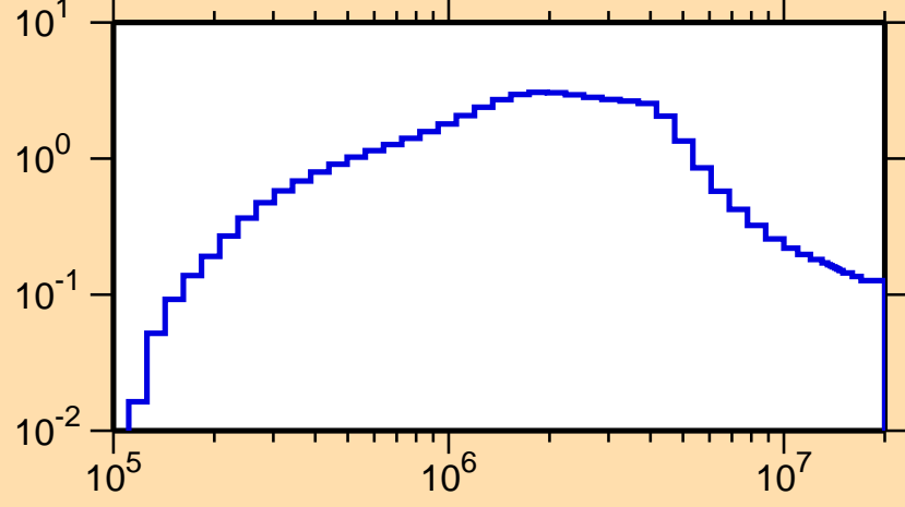
\sigma vs. E for ^{235}\text{Ra}(n,\text{inel.})
