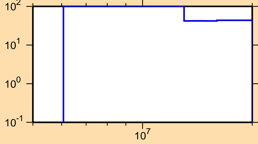
\Delta\sigma/\sigma vs. E for ^{235}\text{Ra}(n,n\text{cont.})
