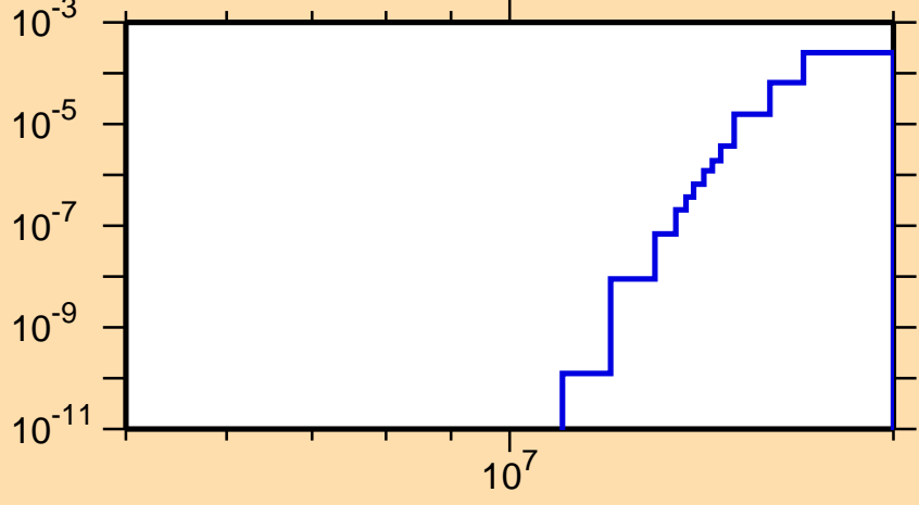
\sigma vs. E for ^{235}\text{Ra}(n,d)
