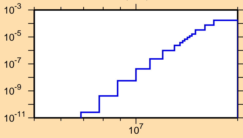
\sigma vs. E for ^{235}\text{Ra}(n,\alpha)
