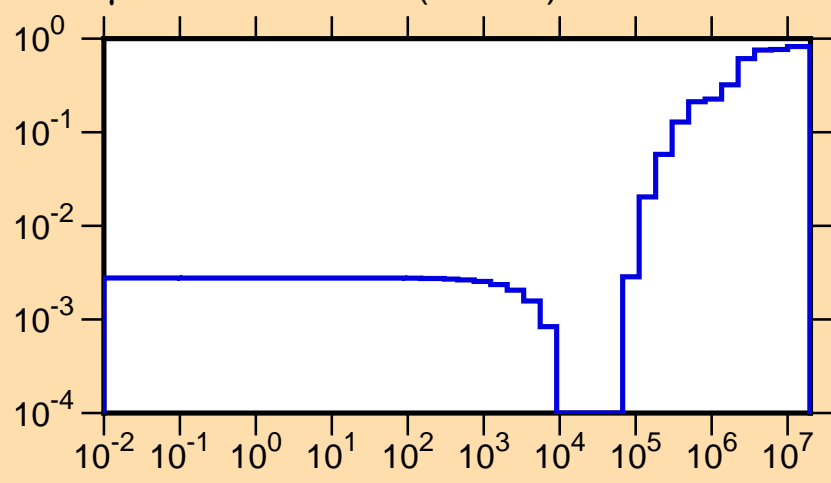
\mu vs. E for ^{235}\text{Ra}(\text{mt251})
