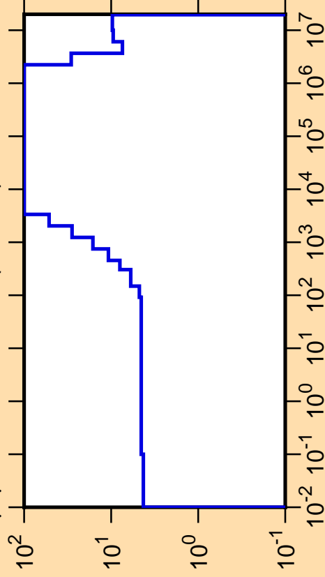
\Delta\mu/\mu vs. E for ^{235}\text{Ra}(\text{mt251})
