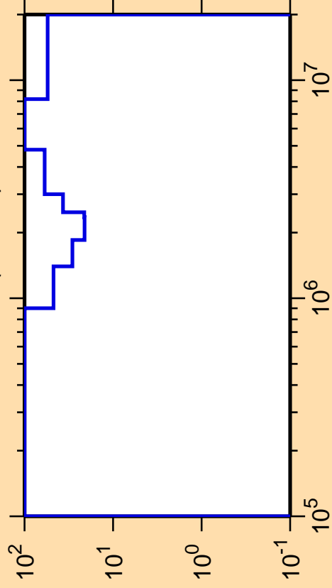
\Delta\sigma/\sigma vs. E for ^{235}\text{Ra}(n,\text{inel.})
