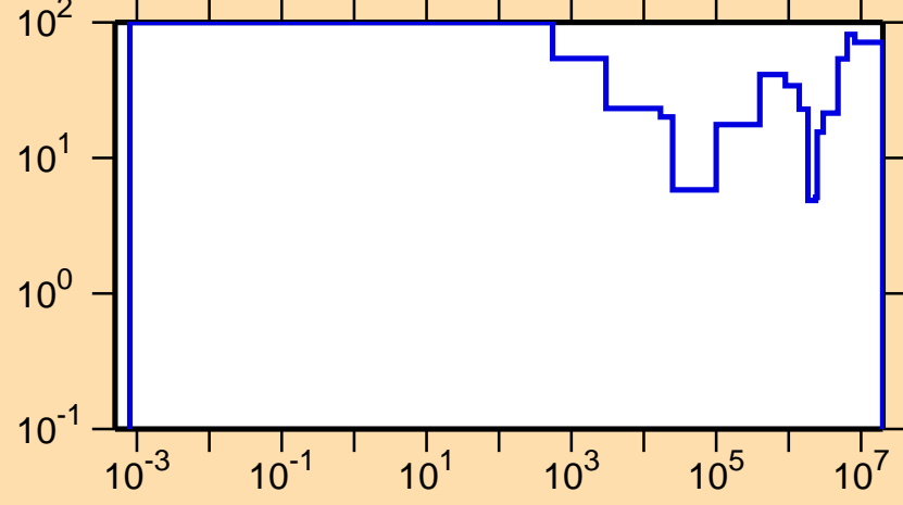
\Delta\sigma/\sigma vs. E for ^{235}\text{Ra}(n,\text{el.})
