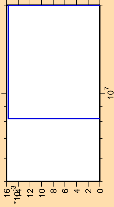
\Delta\sigma/\sigma vs. E for ^{235}\text{Ra}(n,3n\alpha)
