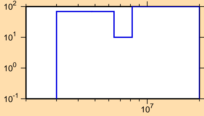
\Delta\sigma/\sigma vs. E for ^{235}\text{Ra}(n,2n)
