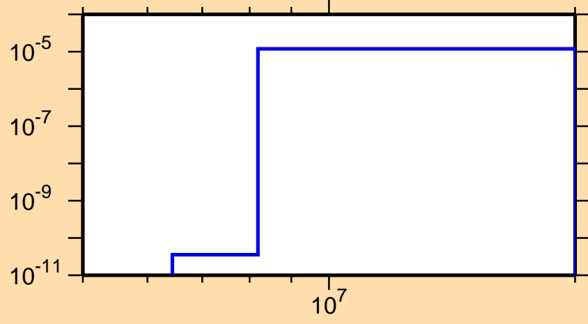
\sigma vs. E for ^{235}\text{Ra}(n,\alpha)
