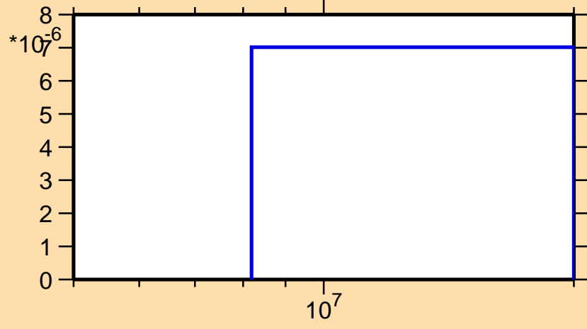
\sigma vs. E for ^{235}\text{Ra}(n,d)
