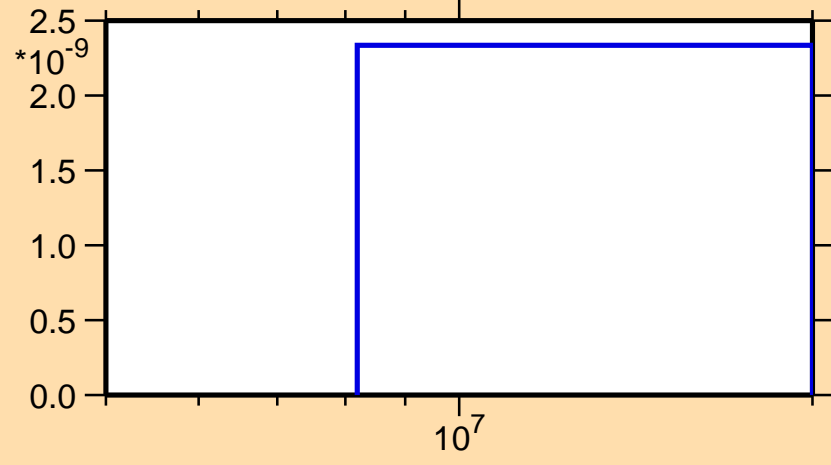
\sigma vs. E for ^{235}\text{Ra}(n,2n\alpha)
