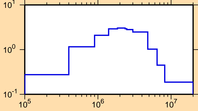
\sigma vs. E for ^{235}\text{Ra}(n,\text{inel.})
