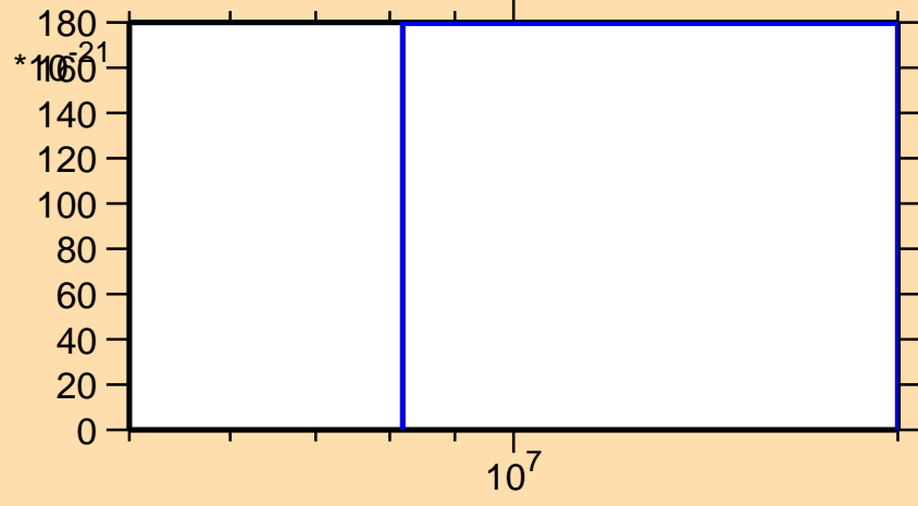
\sigma vs. E for ^{235}\text{Ra}(\text{mt } 42)
