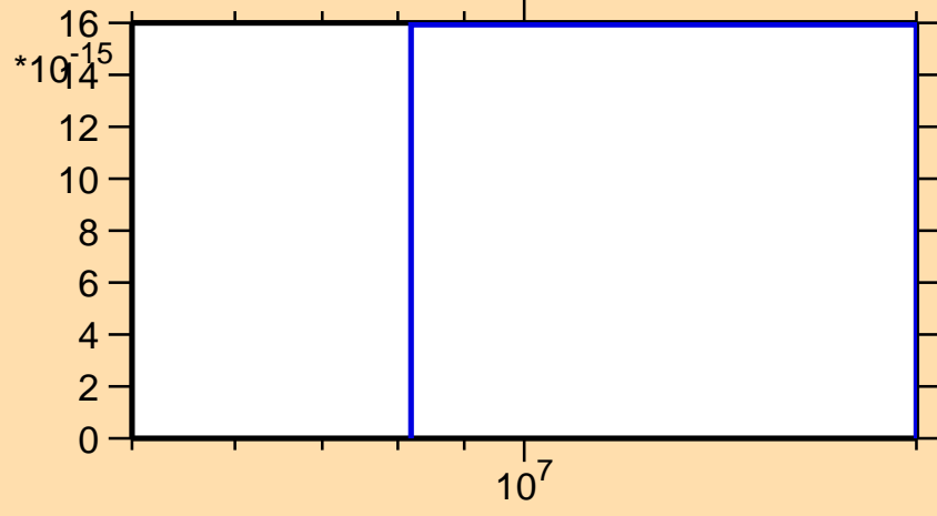
\sigma vs. E for ^{235}\text{Ra}(n,3n\alpha)
