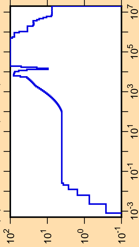
\Delta\mu/\mu vs. E for ^{75}\text{Rb}(\text{mt251})
