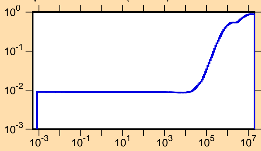
\mu vs. E for ^{75}\text{Rb}(\text{mt251})
