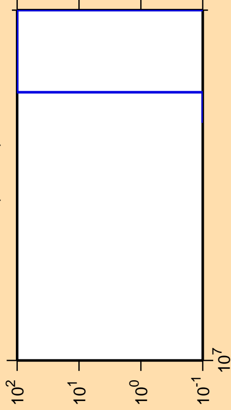
\Delta\sigma/\sigma vs. E for ^{75}\text{Rb} (mt 34)
