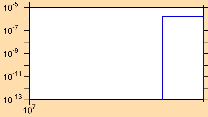
\sigma vs. E for ^{75}\text{Rb}(n,2np)
