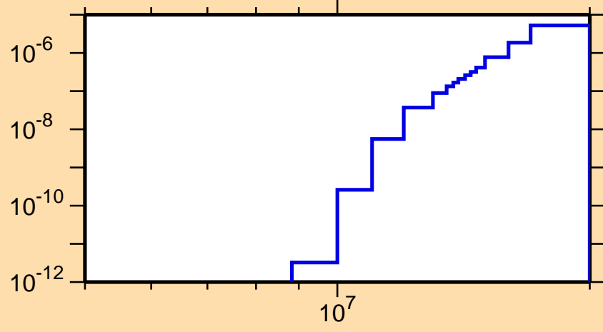
\sigma vs. E for ^{75}\text{Rb}(\text{mt117})
