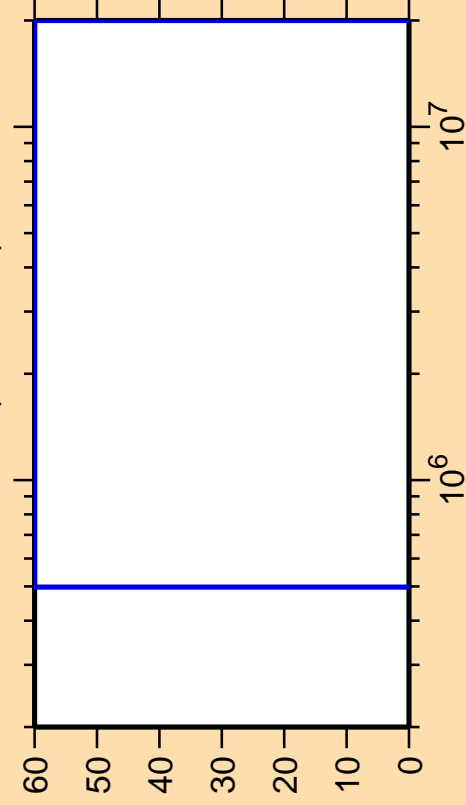
\Delta\sigma/\sigma vs. E for ^{75}\text{Rb}(n,\text{ncont.})
