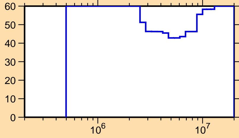
\Delta\sigma/\sigma vs. E for ^{75}\text{Rb}(n,\text{inel.})
