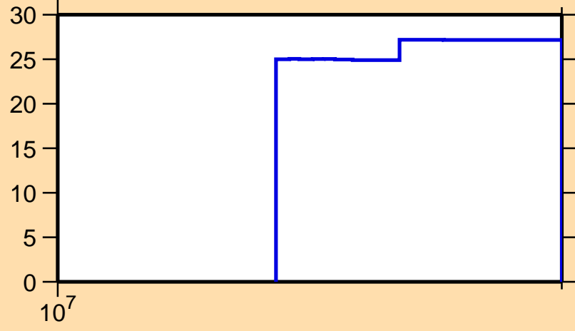
\Delta\sigma/\sigma vs. E for ^{75}\text{Rb}(n,\text{el.})
