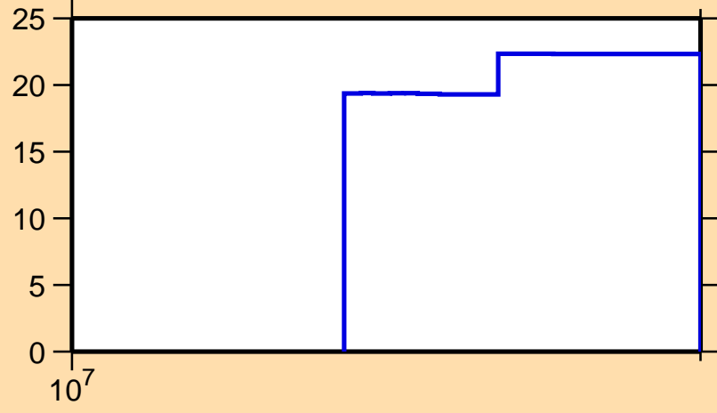
\Delta\sigma/\sigma vs. E for ^{75}\text{Rb}(n,\text{nonel.})
