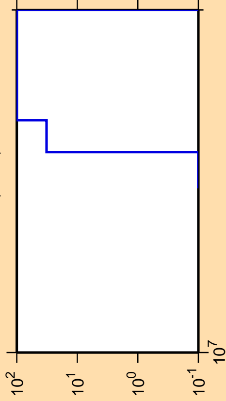
\Delta\sigma/\sigma vs. E for ^{75}\text{Rb}(n,nd)
