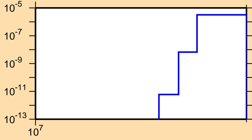
\sigma vs. E for ^{75}\text{Rb}(n,\text{pt})
