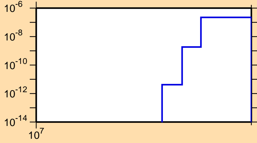
\sigma vs. E for ^{75}\text{Rb}(n,nd)
