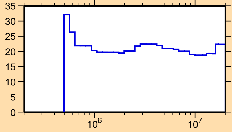
\Delta\sigma/\sigma vs. E for ^{75}\text{Rb}(n,n\text{onel.})
