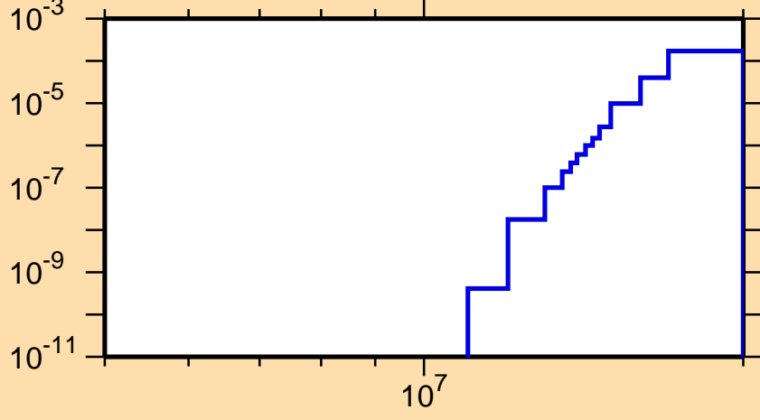
\sigma vs. E for ^{75}\text{Rb} (mt 45)
