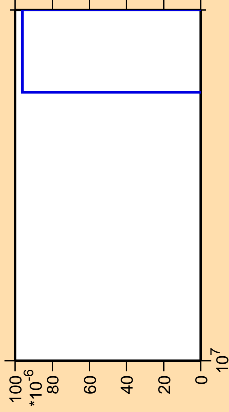
\Delta\sigma/\sigma vs. E for ^{75}\text{Rb}(n,nt)
