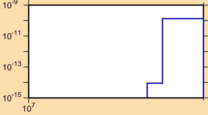
\sigma vs. E for ^{75}\text{Rb} (mt 34)
