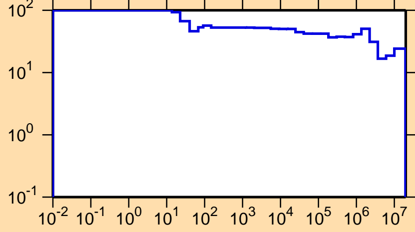
\Delta\sigma/\sigma vs. E for ^{75}\text{Rb}(n,\text{el.})
