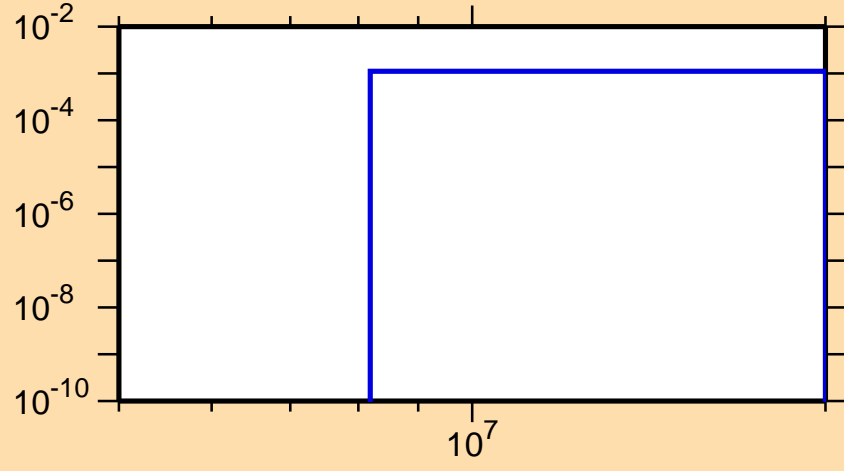
\sigma vs. E for ^{75}\text{Rb}(n,\alpha)
