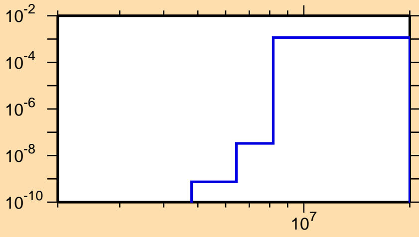
\sigma vs. E for ^{75}\text{Rb}(n,\text{He}3)
