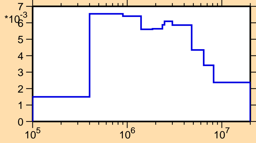
\sigma vs. E for ^{75}\text{Rb}(n,n_2)
