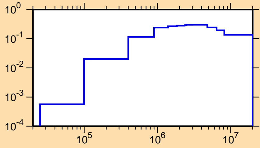
\sigma vs. E for ^{75}\text{Rb}(n,\text{inel.})
