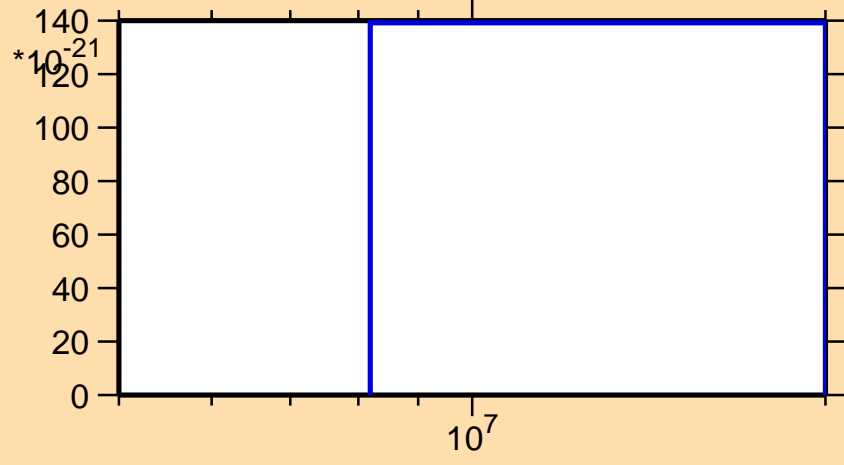
\sigma vs. E for ^{75}\text{Rb}(n,nt)
