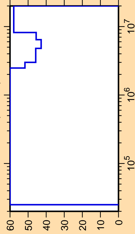
\Delta\sigma/\sigma vs. E for ^{75}\text{Rb}(n,\text{inel.})
