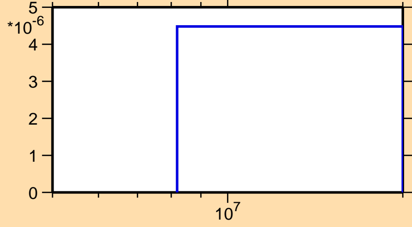
\sigma vs. E for ^{75}\text{Rb}(n,2n)
