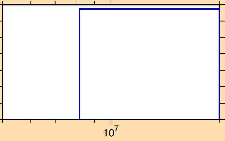
\sigma vs. E for ^{75}\text{Rb}(n,\text{pd})
