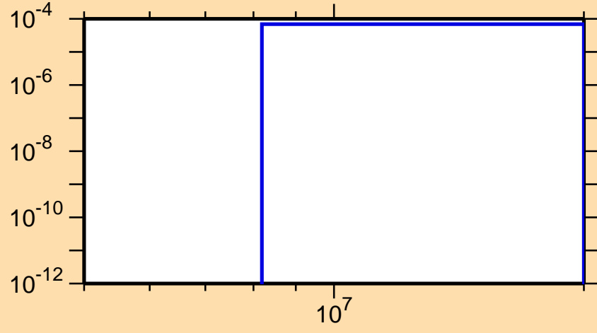
\sigma vs. E for ^{75}\text{Rb}(n,t)
