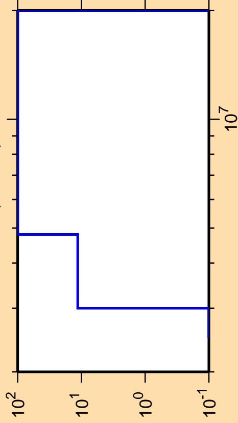
\Delta\sigma/\sigma vs. E for ^{75}\text{Rb}(n,\text{He}3)
