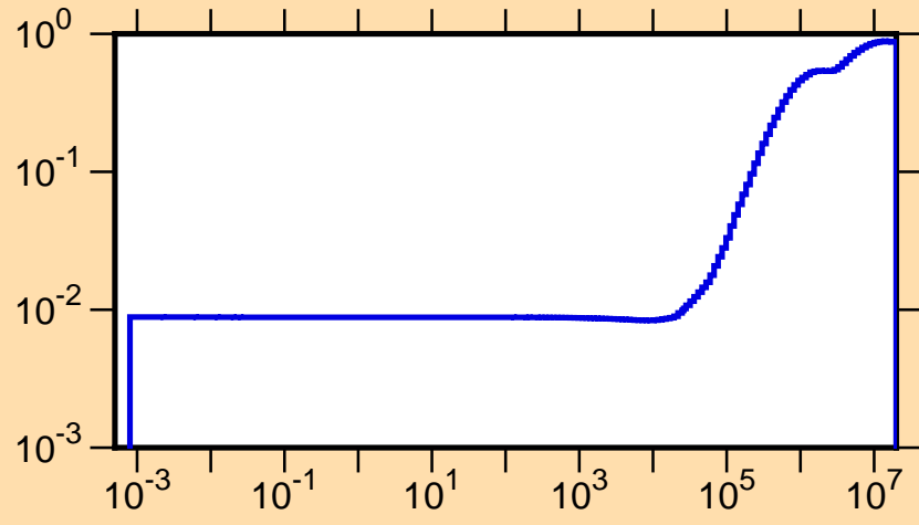
\mu vs. E for ^{76}\text{Rb}(\text{mt251})
