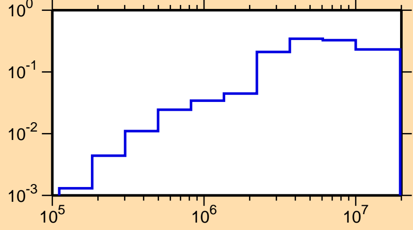
\sigma vs. E for ^{76}\text{Rb}(n,\text{inel.})
