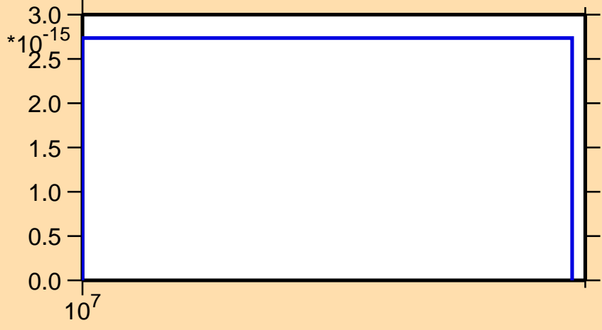
\sigma vs. E for ^{76}\text{Rb}(n,2n\alpha)
