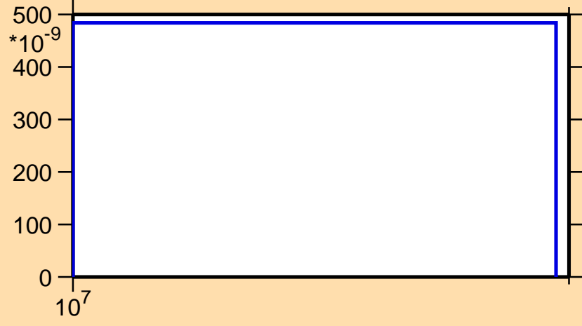
\sigma vs. E for ^{76}\text{Rb}(n,\text{pt})
