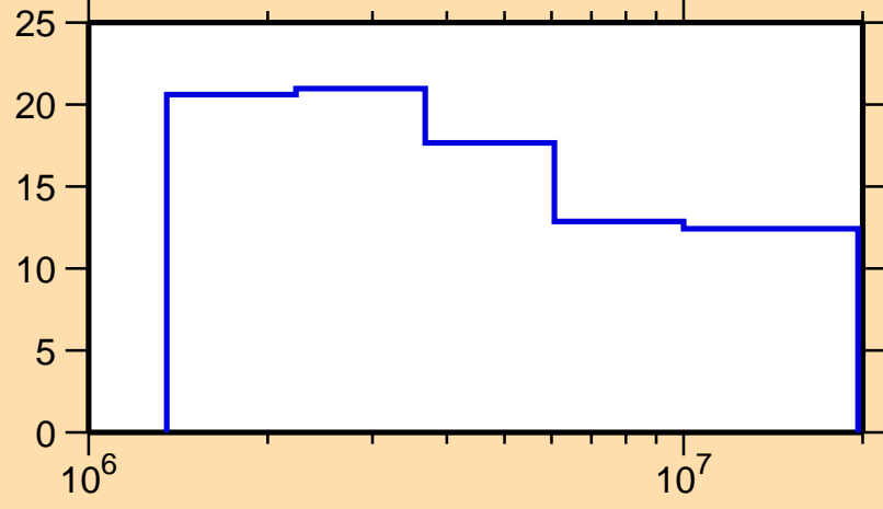
\Delta\sigma/\sigma vs. E for ^{76}\text{Rb}(n,n\text{nonel.})
