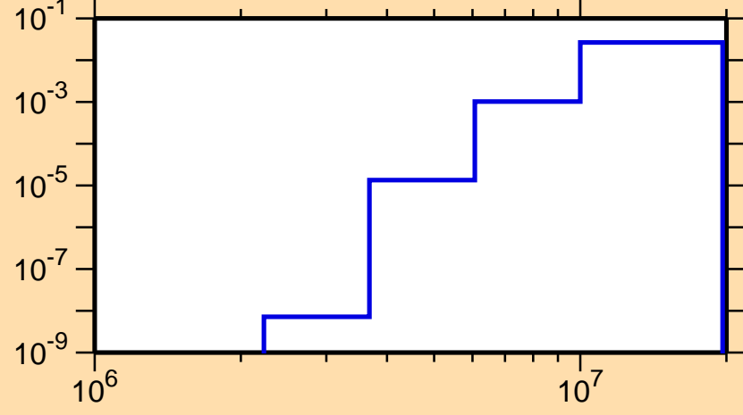
\sigma vs. E for ^{76}\text{Rb}(n,d)
