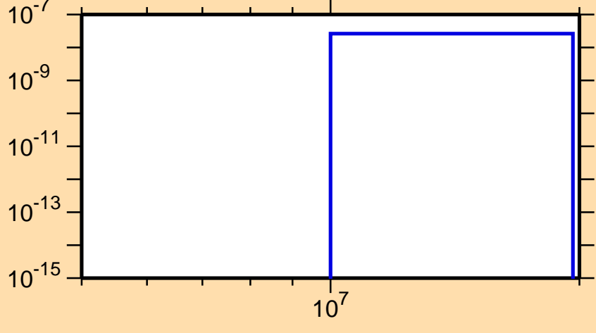
\sigma vs. E for ^{76}\text{Rb}(\text{mt117})
