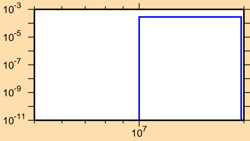
\sigma vs. E for ^{76}\text{Rb}(n,pd)
