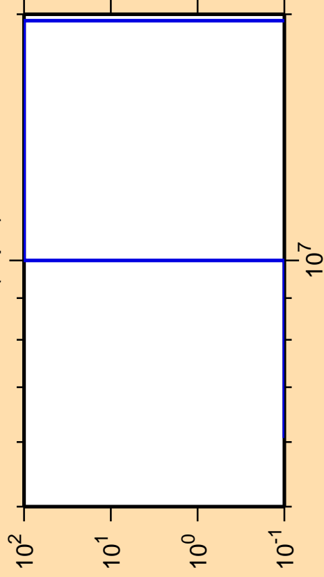
\Delta\sigma/\sigma vs. E for ^{76}\text{Rb}(n,pd)
