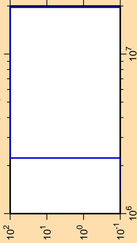
\Delta\sigma/\sigma vs. E for ^{76}\text{Rb}(n,d)
