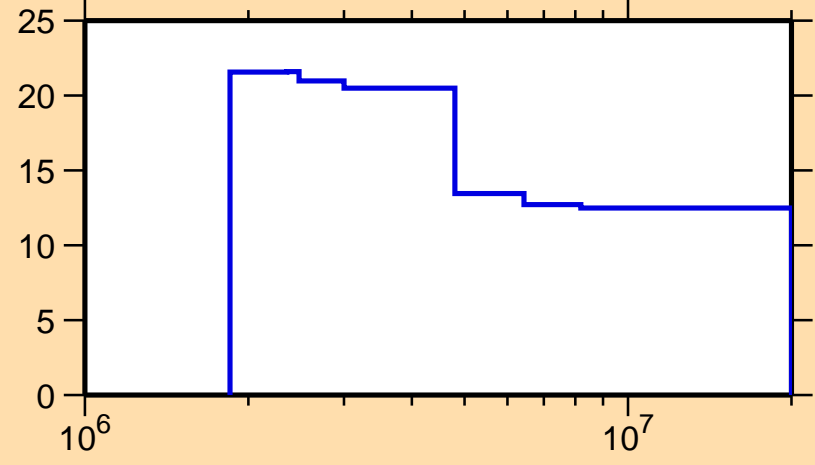
\Delta\sigma/\sigma vs. E for ^{76}\text{Rb}(n,n\text{onel.})
