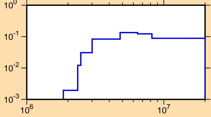
\sigma vs. E for ^{76}\text{Rb}(n,n\text{cont.})
