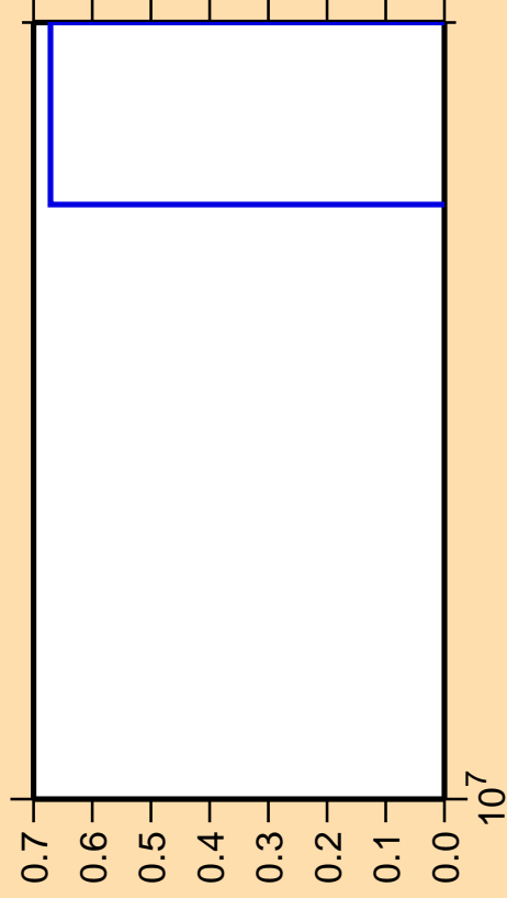
\Delta\sigma/\sigma vs. E for ^{77}\text{Rb}(n,nt)
