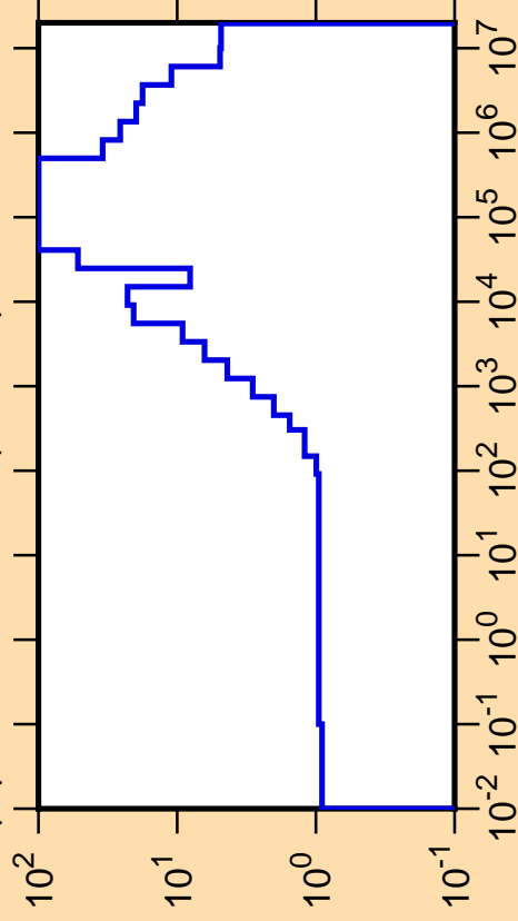
\Delta\mu/\mu vs. E for ^{77}\text{Rb}(\text{mt251})
