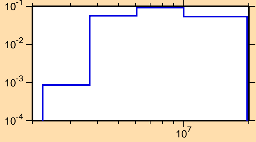
\sigma vs. E for ^{77}\text{Rb}(n,n\text{cont.})
