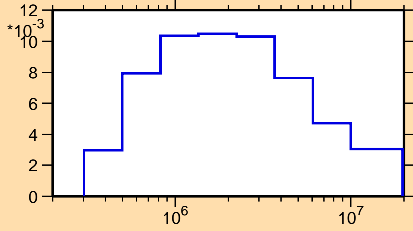
\sigma vs. E for ^{77}\text{Rb}(n,n_3)
