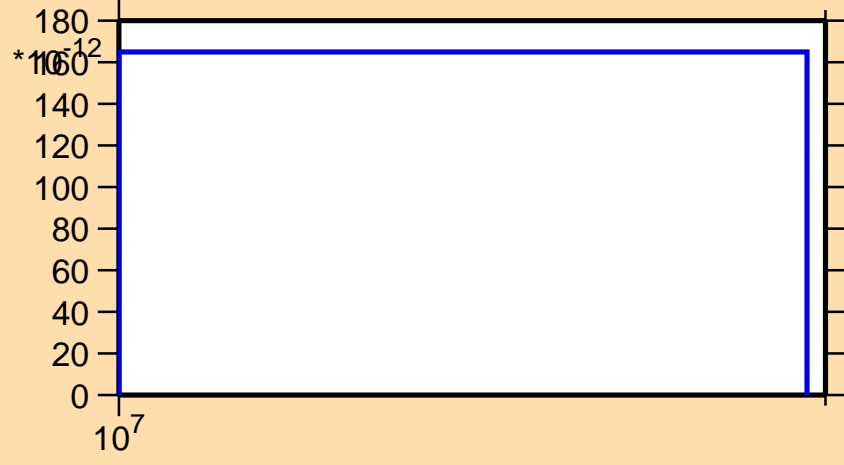
\sigma vs. E for ^{77}\text{Rb}(n,pt)
