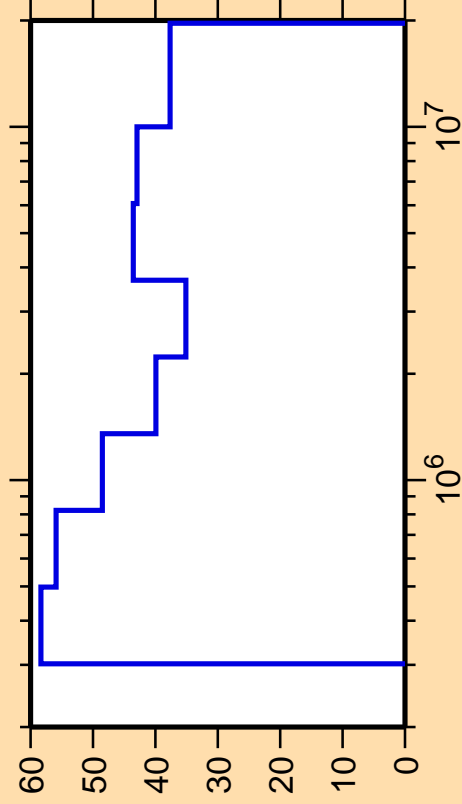
\Delta\sigma/\sigma vs. E for ^{77}\text{Rb}(n,n_3)
