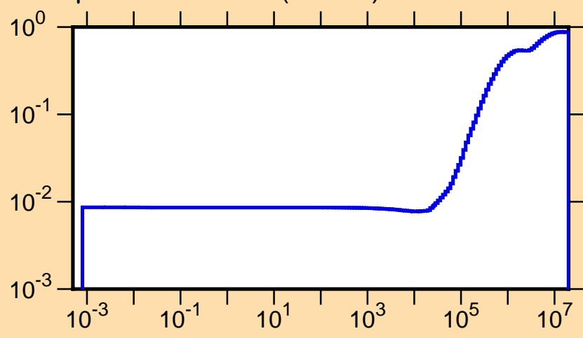
\mu vs. E for ^{78}\text{Rb}(\text{mt251})
