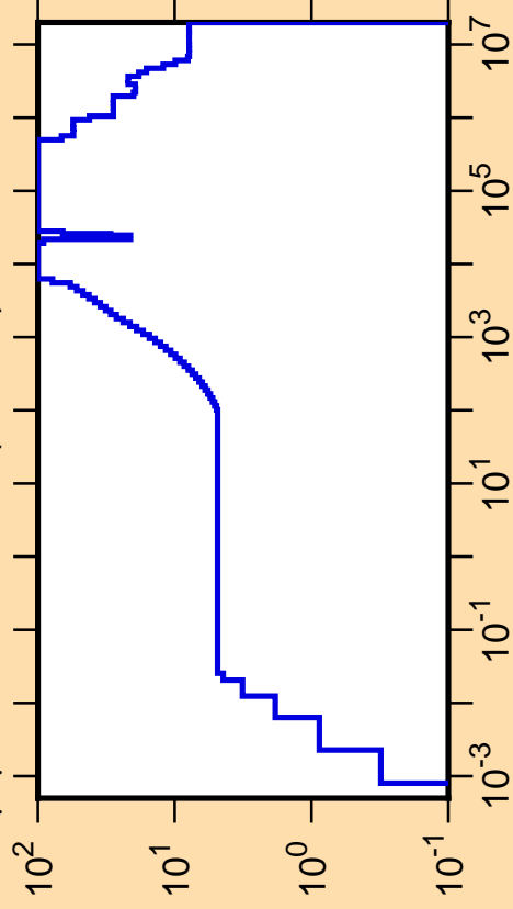
\Delta\mu/\mu vs. E for ^{78}\text{Rb}(\text{mt251})
