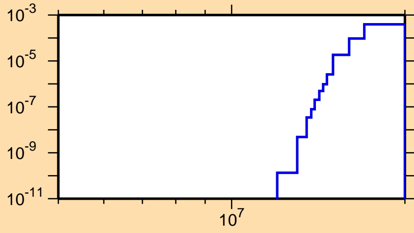
\sigma vs. E for ^{78}\text{Rb}(n,pd)
