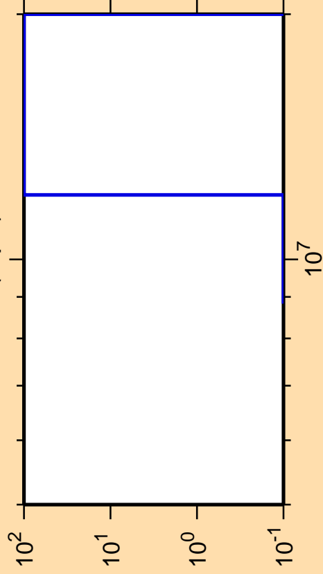
\Delta\sigma/\sigma vs. E for ^{78}\text{Rb}(n,pd)
