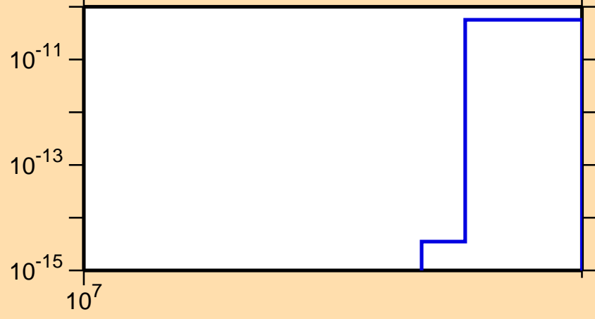
\sigma vs. E for ^{78}\text{Rb}(n,2n\alpha)
