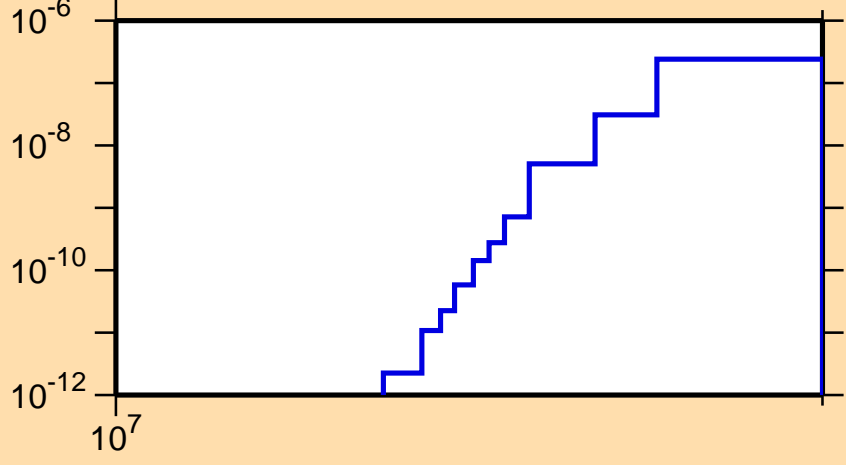
\sigma vs. E for ^{78}\text{Rb}(\text{mt117})
