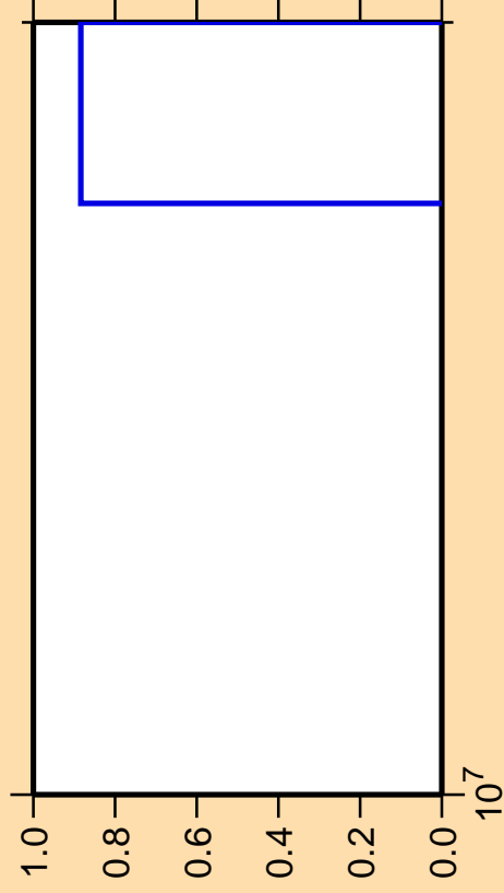
\Delta\sigma/\sigma vs. E for ^{78}\text{Rb}(n,nt)
