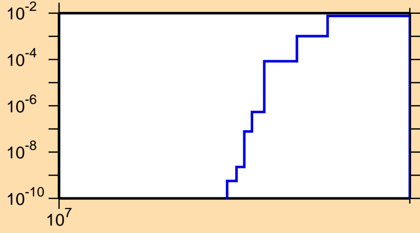
\sigma vs. E for ^{78}\text{Rb}(n,2np)
