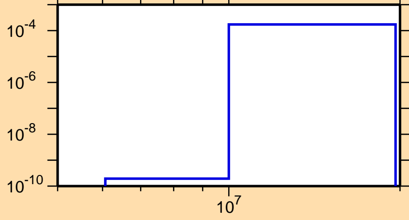
\sigma vs. E for ^{78}\text{Rb}(n,\text{He}3)
