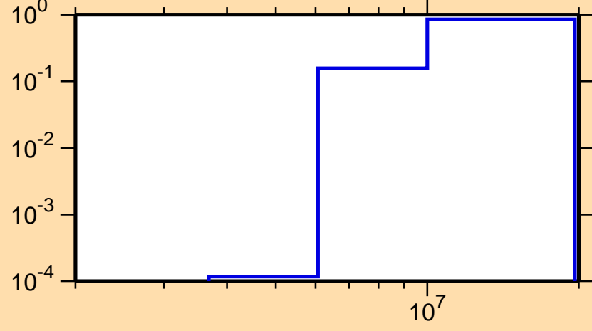
\sigma vs. E for ^{78}\text{Rb}(n,np)
