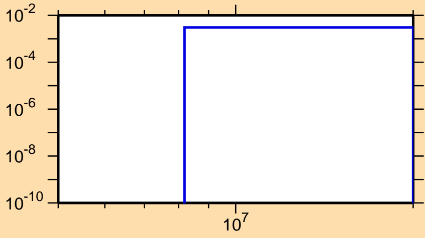
\sigma vs. E for ^{78}\text{Rb}(n,\alpha)
