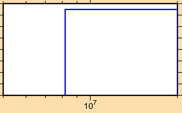
\sigma vs. E for ^{78}\text{Rb}(n,2n)
