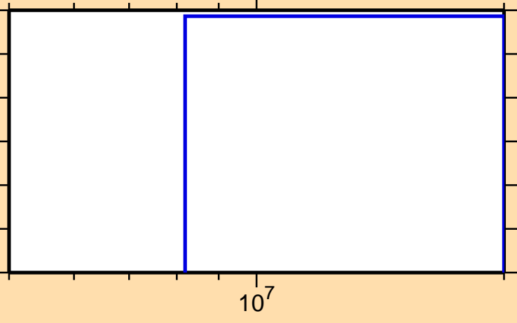
\sigma vs. E for ^{78}\text{Rb}(n,\text{pt})
