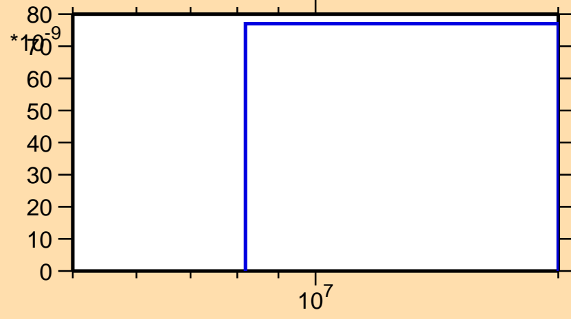
\sigma vs. E for ^{78}\text{Rb} (mt 45)
