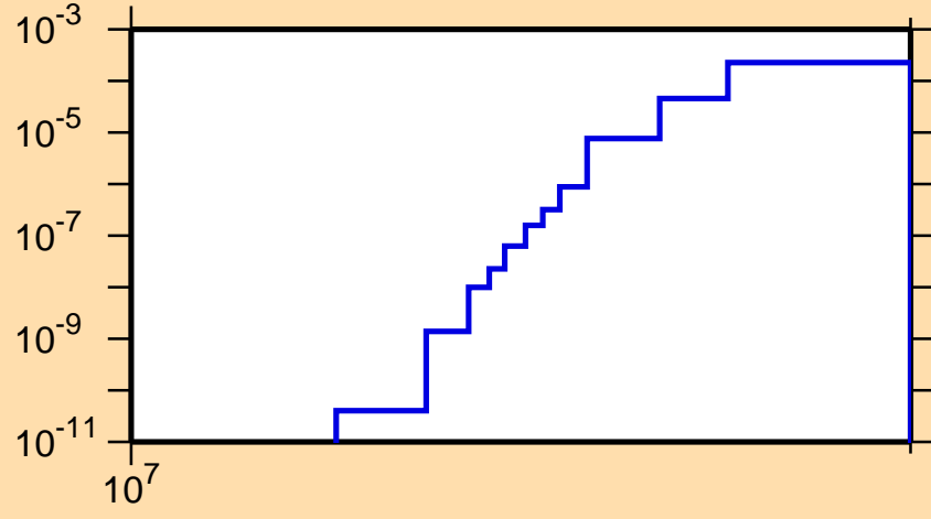
\sigma vs. E for ^{78}\text{Rb}(n,pd)
