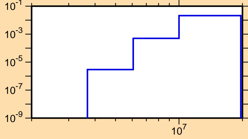
\sigma vs. E for ^{78}\text{Rb}(n,d)
