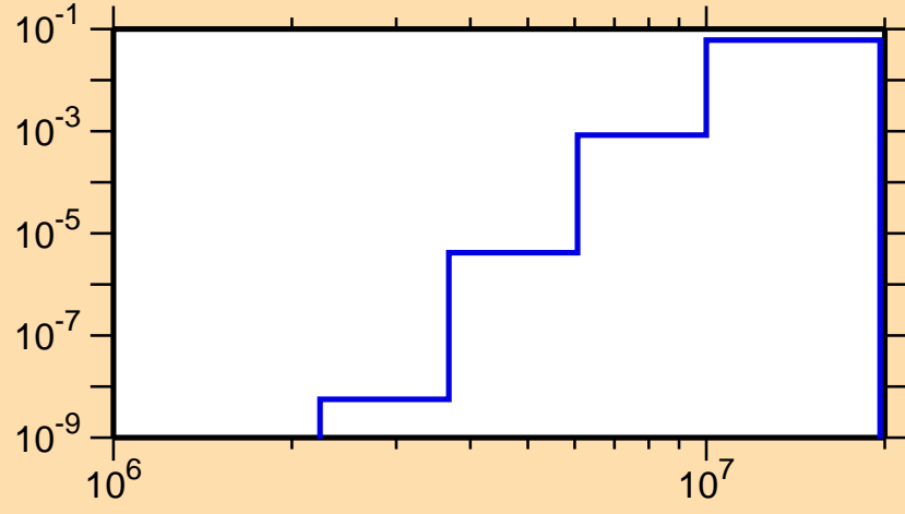
\sigma vs. E for ^{78}\text{Rb}(n,p\alpha)
