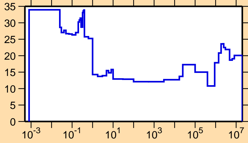
\Delta\sigma/\sigma vs. E for ^{78}\text{Rb}(n,p)
