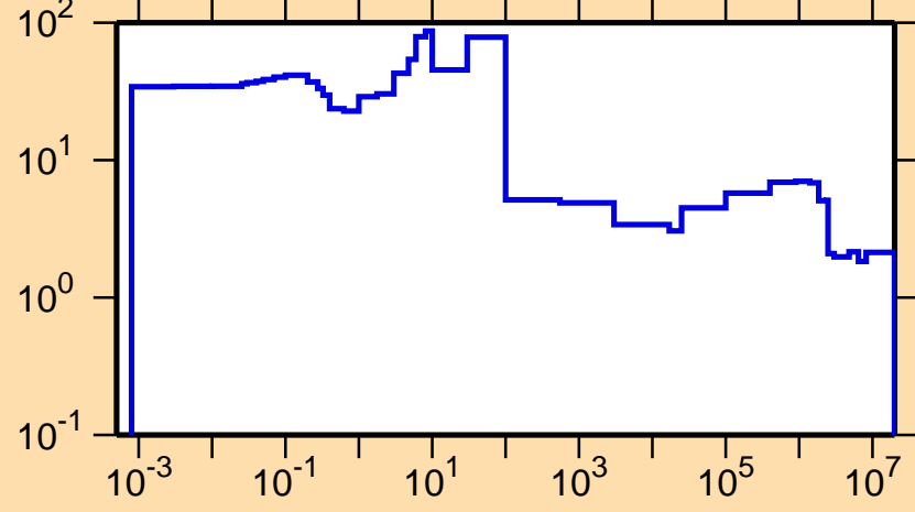
\Delta\sigma/\sigma vs. E for ^{78}\text{Rb}(n,\text{tot.})
