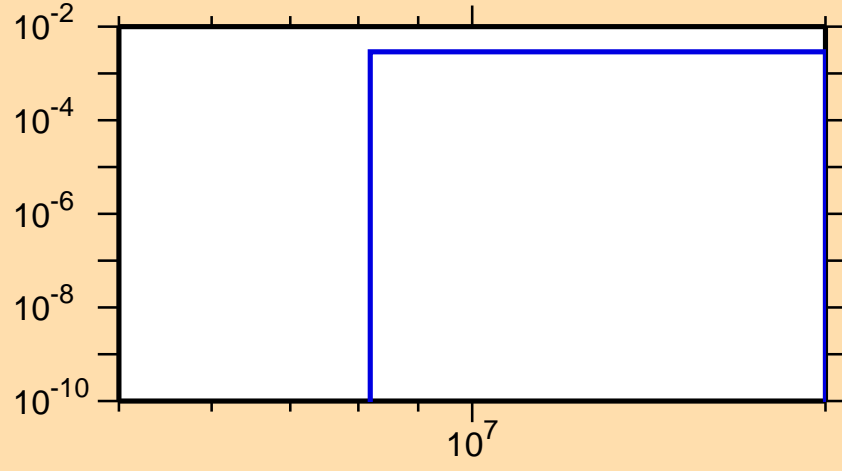
\sigma vs. E for ^{78}\text{Rb}(n,\alpha)
