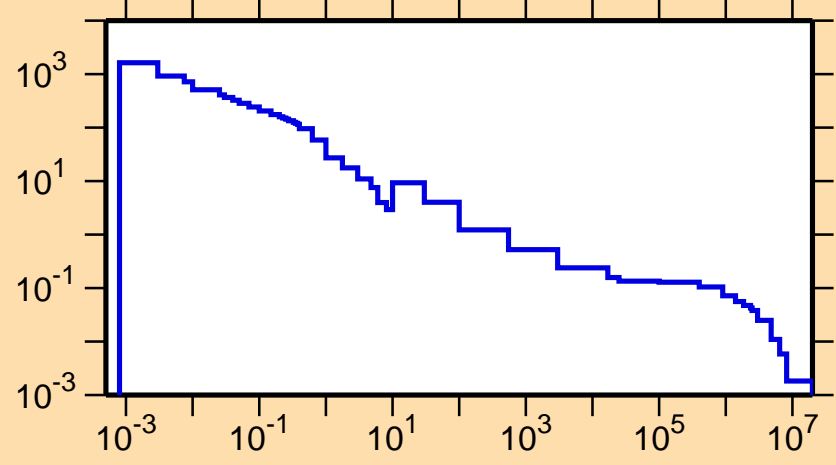
\sigma vs. E for ^{78}\text{Rb}(n,\gamma)
