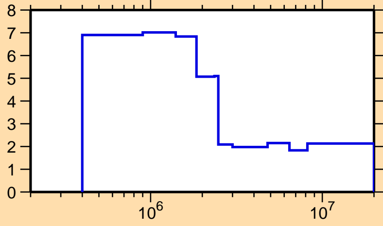
\Delta\sigma/\sigma vs. E for ^{78}\text{Rb}(n,tot.)
