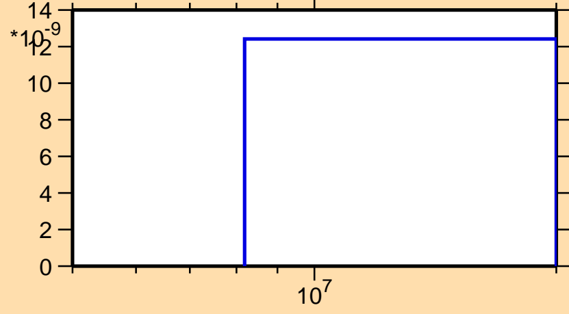
\sigma vs. E for ^{78}\text{Rb}(n,pt)
