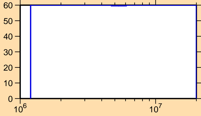
\Delta\sigma/\sigma vs. E for ^{79}\text{Rb}(n,ncont.)
