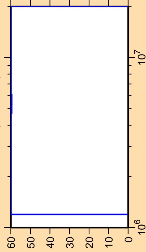
\Delta\sigma/\sigma vs. E for ^{79}\text{Rb}(n,n\text{cont.})
