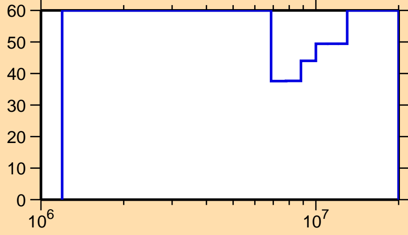
\Delta\sigma/\sigma vs. E for ^{79}\text{Rb}(n,n_1)
