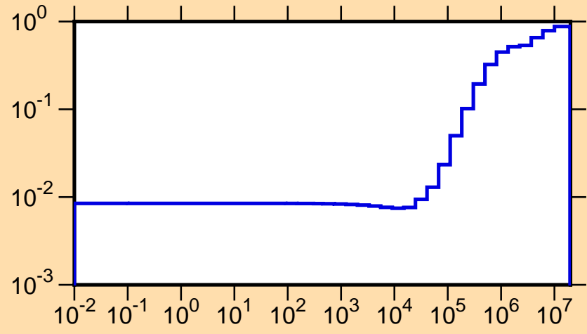
\mu vs. E for ^{79}\text{Rb}(\text{mt251})
