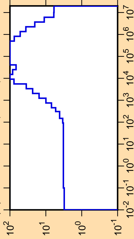
\Delta\mu/\mu vs. E for ^{79}\text{Rb}(\text{mt251})
