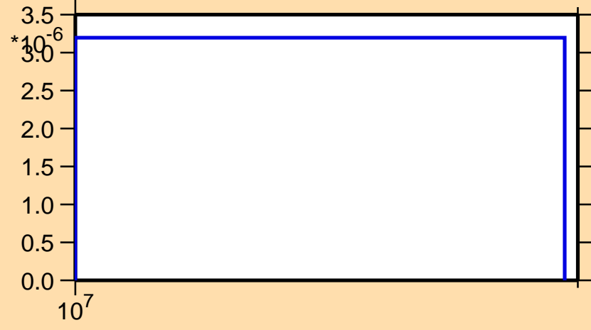
\sigma vs. E for ^{79}\text{Rb}(n,pd)
