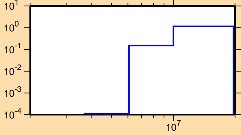
\sigma vs. E for ^{79}\text{Rb}(n,np)
