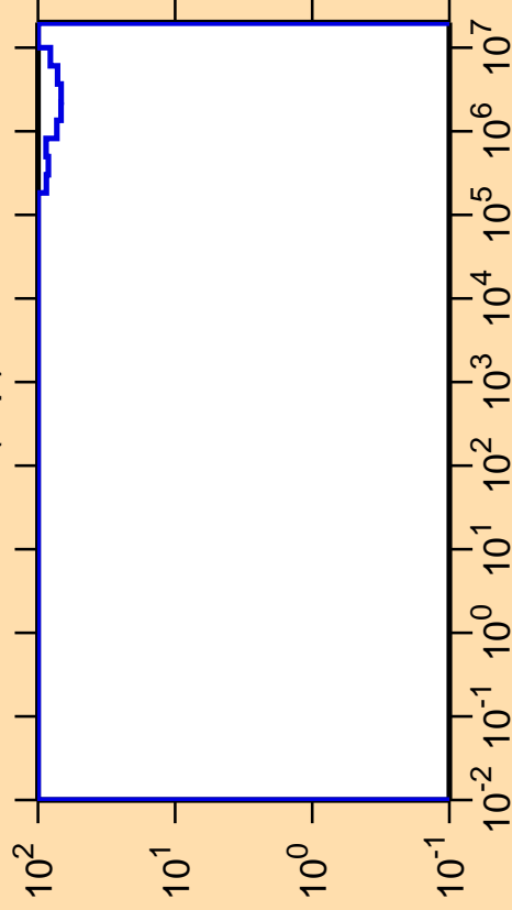
\Delta\sigma/\sigma vs. E for ^{79}\text{Rb}(n,p)
