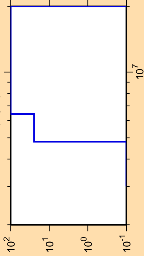
\Delta\sigma/\sigma vs. E for ^{79}\text{Rb}(n,p\alpha)
