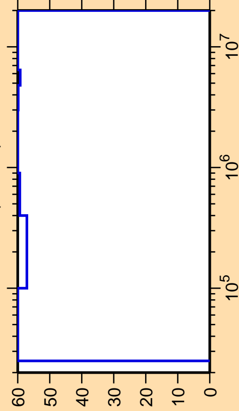
\Delta\sigma/\sigma vs. E for ^{79}\text{Rb}(n,\text{inel.})
