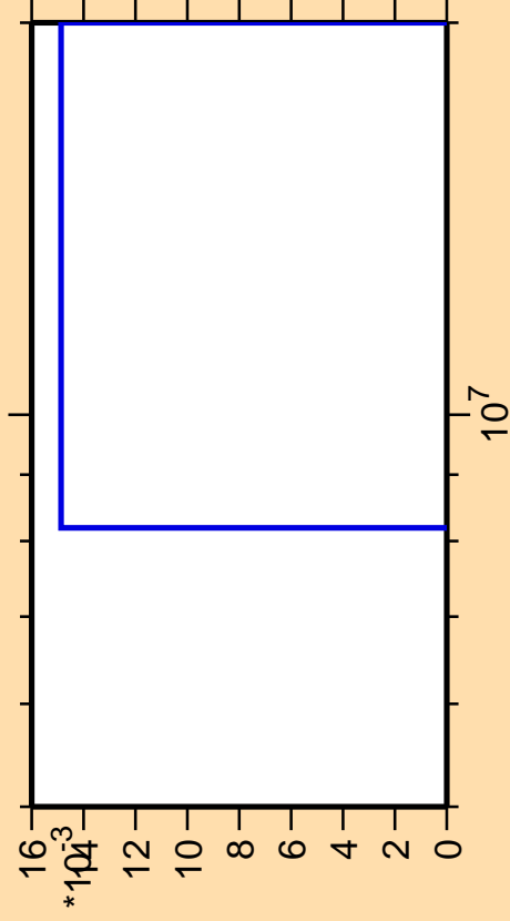
\Delta\sigma/\sigma vs. E for ^{79}\text{Rb} (mt 34)
