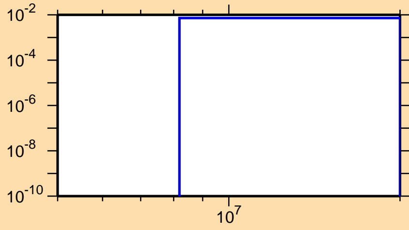
\sigma vs. E for ^{79}\text{Rb}(n,\alpha)
