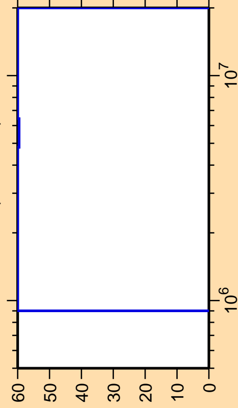
\Delta\sigma/\sigma vs. E for ^{79}\text{Rb}(n,\text{ncont.})
