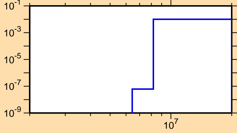
\sigma vs. E for ^{79}\text{Rb}(n,p\alpha)
