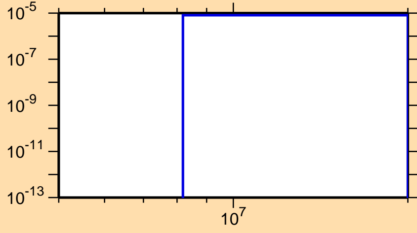
\sigma vs. E for ^{79}\text{Rb}(n,\text{He}3)
