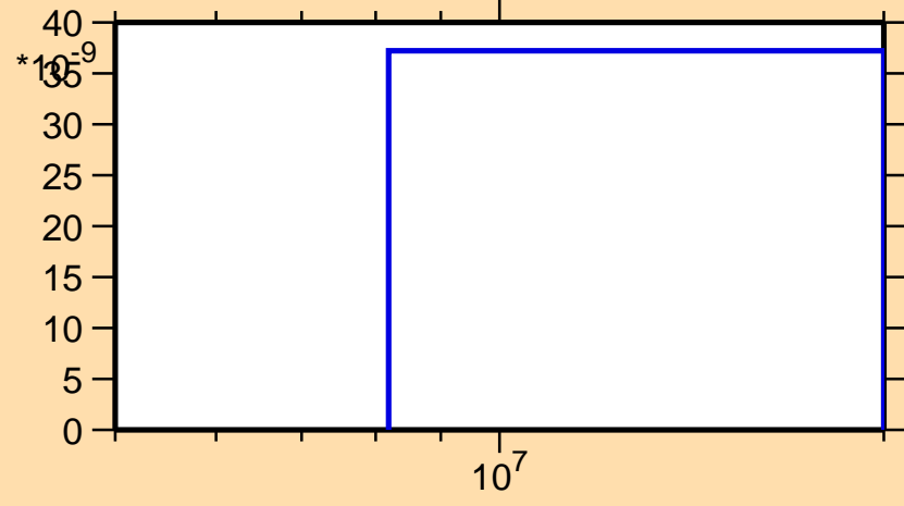
\sigma vs. E for ^{79}\text{Rb} (mt 45)
