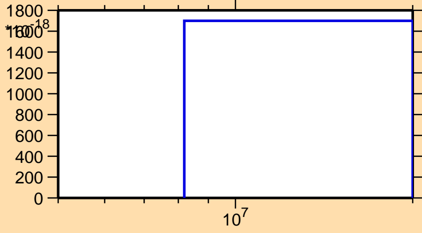
\sigma vs. E for ^{79}\text{Rb} (mt 34)
