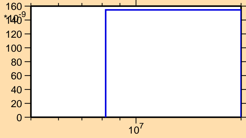
\sigma vs. E for ^{79}\text{Rb}(n,nd)
