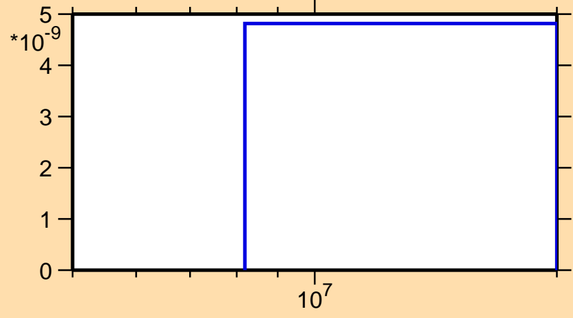
\sigma vs. E for ^{79}\text{Rb}(\text{mt117})
