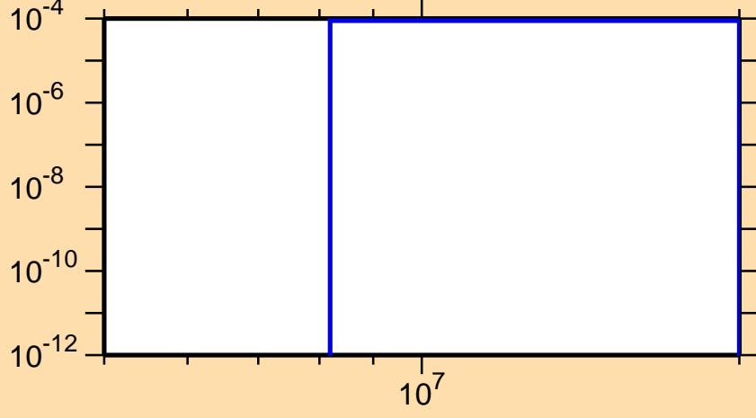
\sigma vs. E for ^{79}\text{Rb}(n,t)
