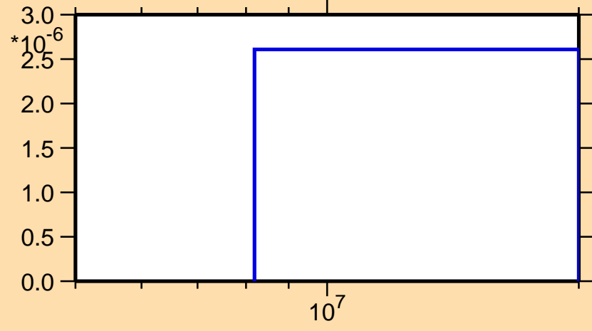
\sigma vs. E for ^{79}\text{Rb}(n,\text{pd})
