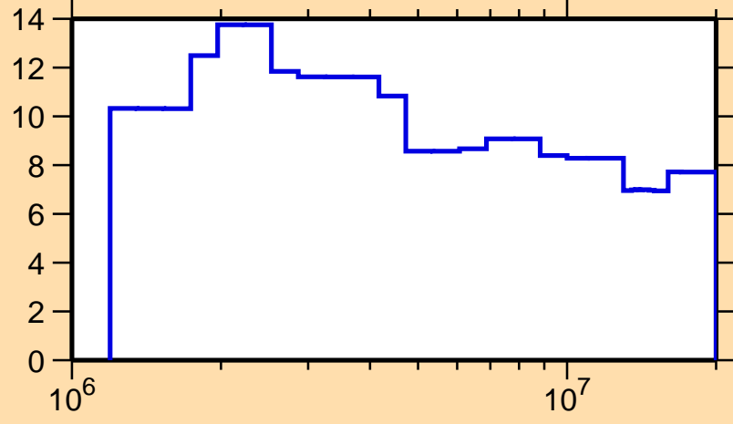
\Delta\sigma/\sigma vs. E for ^{81}\text{Rb}(n,n\text{onel.})
