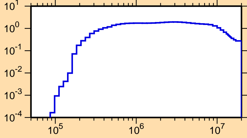
\sigma vs. E for ^{81}\text{Rb}(n,\text{inel.})
