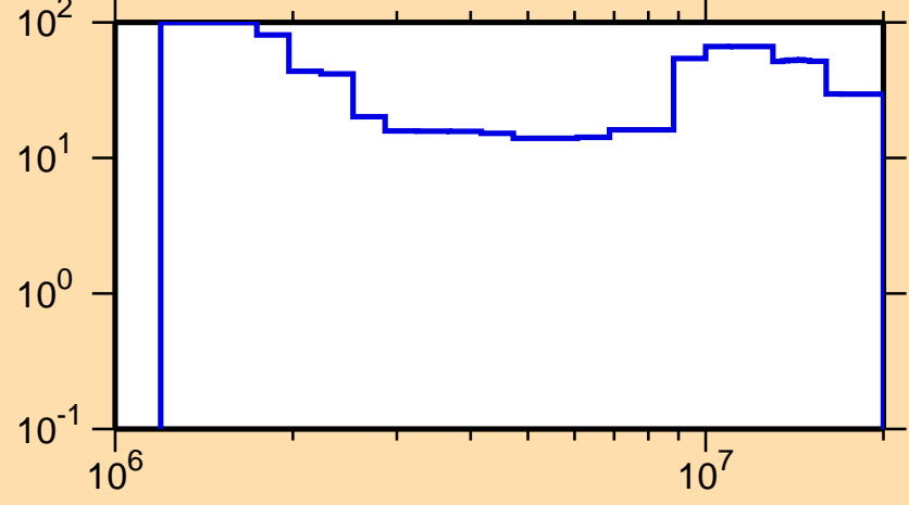
\Delta\sigma/\sigma vs. E for ^{81}\text{Rb}(n,ncont.)
