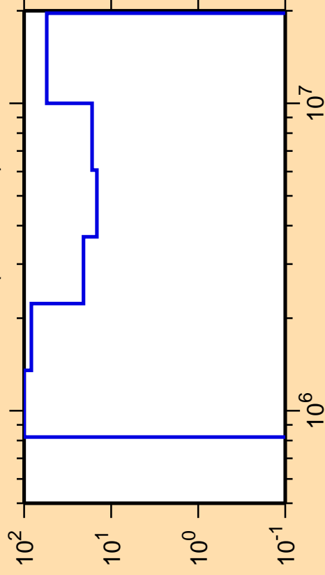
\Delta\sigma/\sigma vs. E for ^{81}\text{Rb}(n,\text{ncont.})
