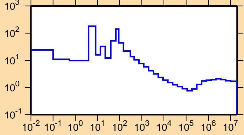
\sigma vs. E for ^{81}\text{Rb}(n,\text{nonel.})
