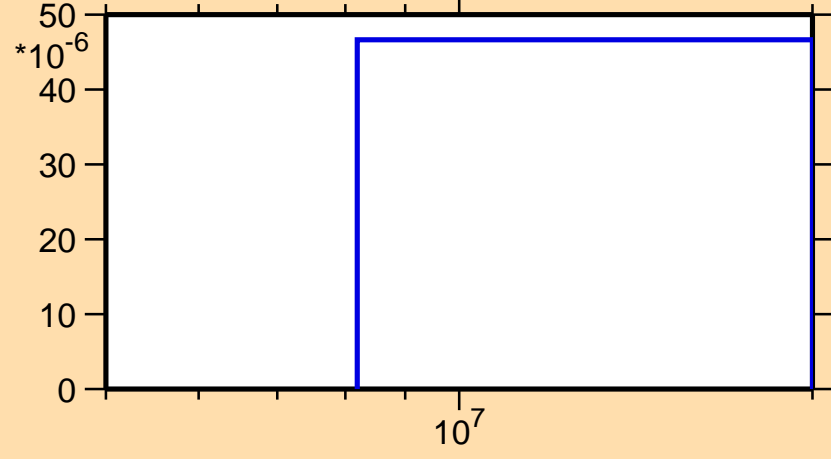
\sigma vs. E for ^{81}\text{Rb}(n,t)
