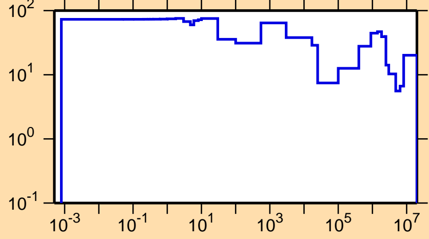
\Delta\sigma/\sigma vs. E for ^{81}\text{Rb}(n,\text{el.})
