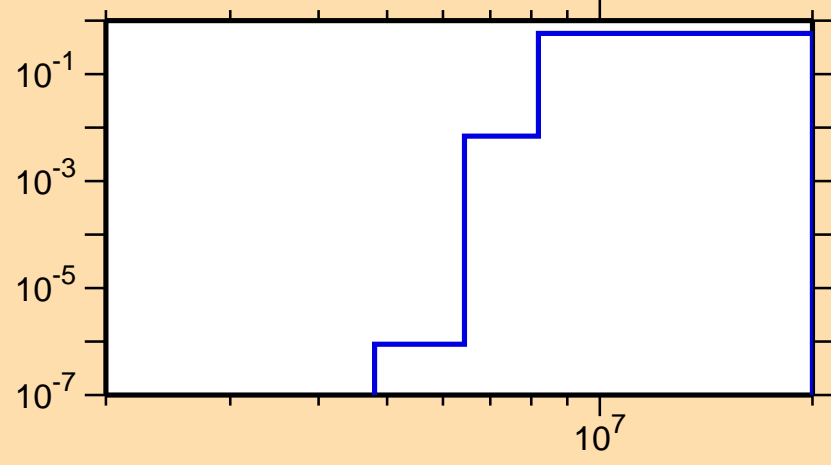
\sigma vs. E for ^{81}\text{Rb}(n,np)
