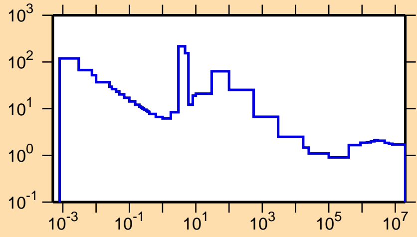
\sigma vs. E for ^{81}\text{Rb}(n,\text{nonel.})
