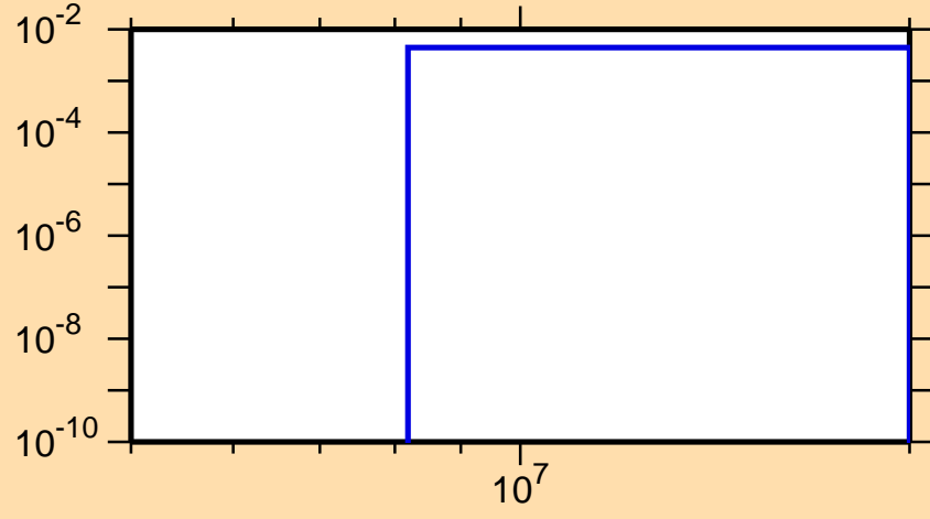
\sigma vs. E for ^{81}\text{Rb}(n,\alpha)
