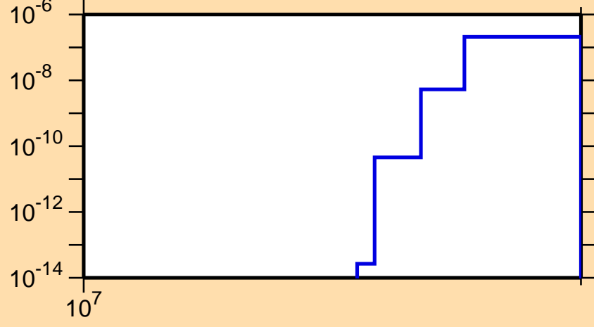
\sigma vs. E for ^{81}\text{Rb}(n,pd)
