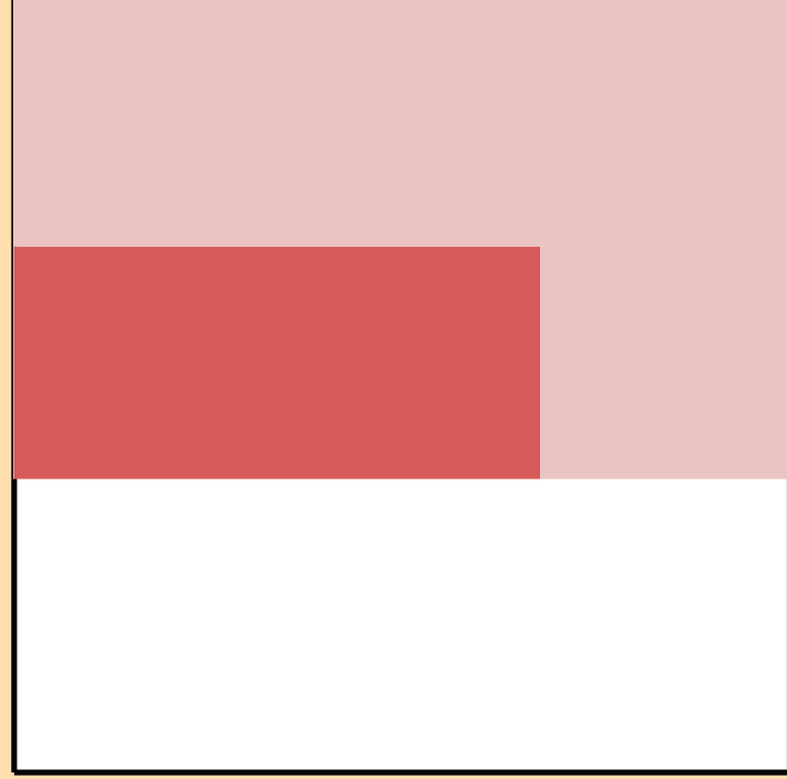
\Delta\sigma/\sigma vs. E for ^{81}\text{Rb}(n,\text{nonel.})
