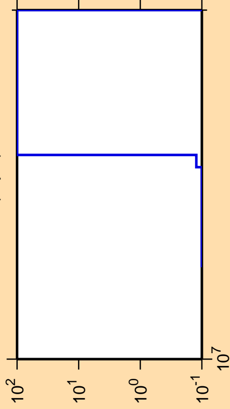
\Delta\sigma/\sigma vs. E for ^{81}\text{Rb}(n,pd)
