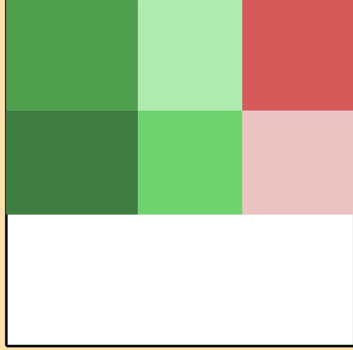
\Delta\sigma/\sigma vs. E for ^{81}\text{Rb}(n,\text{el.})
