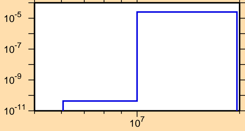
\sigma vs. E for ^{81}\text{Rb}(n,p\alpha)
