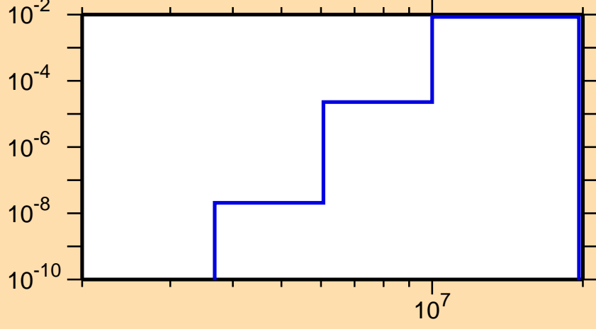
\sigma vs. E for ^{81}\text{Rb}(n,d)
