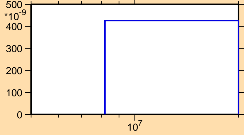
\sigma vs. E for ^{81}\text{Rb}(n,2np)
