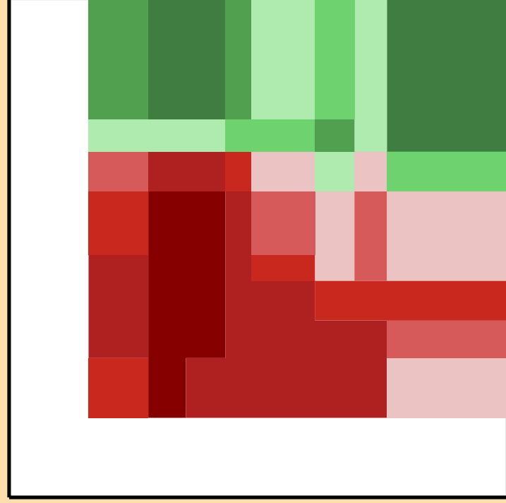
\Delta\sigma/\sigma vs. E for ^{81}\text{Rb}(n,n\text{cont.})
