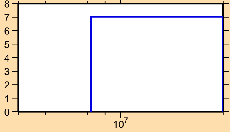
\Delta\sigma/\sigma vs. E for ^{81}\text{Rb}(n,\text{tot.})
