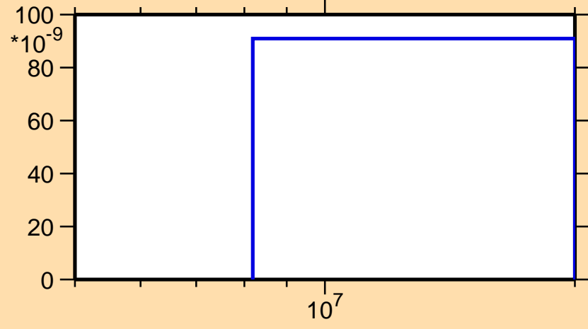
\sigma vs. E for ^{81}\text{Rb}(n,nd)
