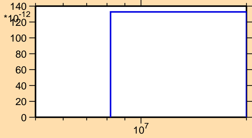
\sigma vs. E for ^{81}\text{Rb} (mt 45)
