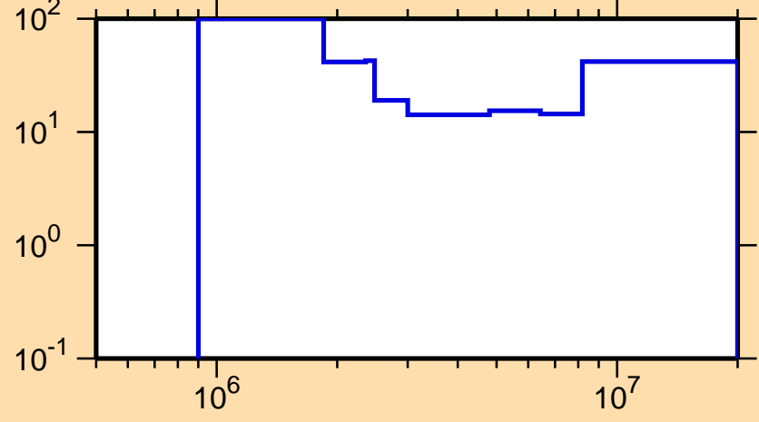
\Delta\sigma/\sigma vs. E for ^{81}\text{Rb}(n,n\text{cont.})
