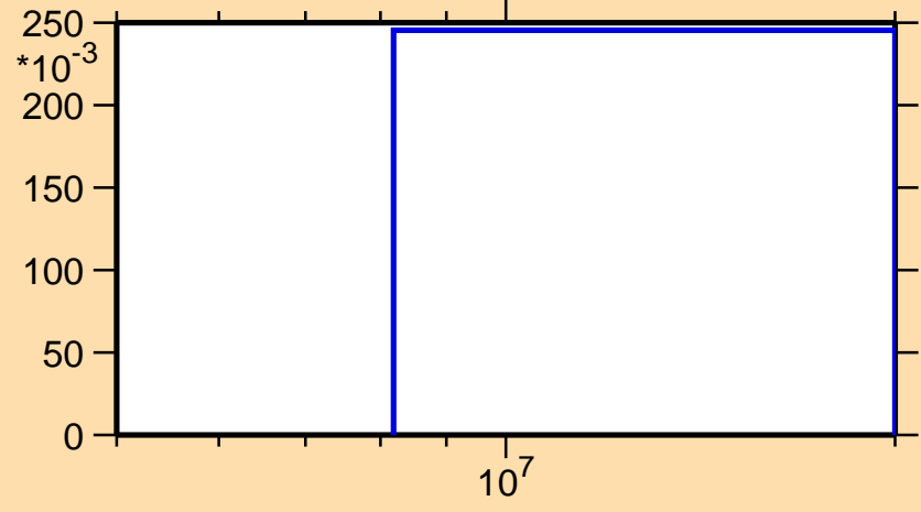
\sigma vs. E for ^{81}\text{Rb}(n,2n)
