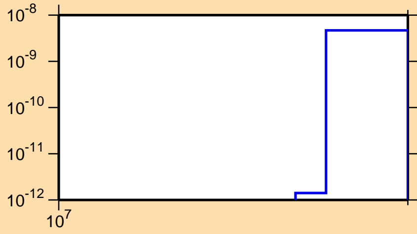
\sigma vs. E for ^{82}\text{Rb}(n,pd)
