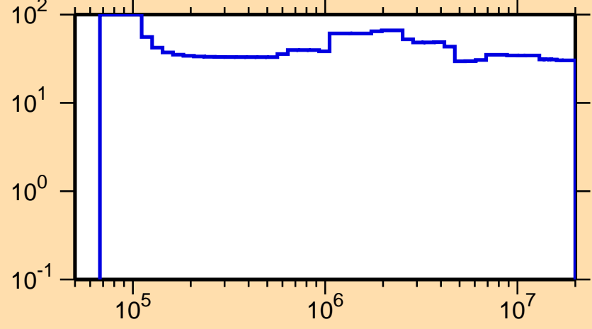
\Delta\sigma/\sigma vs. E for ^{82}\text{Rb}(n,n_1)
