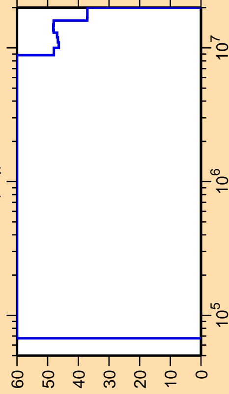
\Delta\sigma/\sigma vs. E for ^{82}\text{Rb}(n,\gamma)
