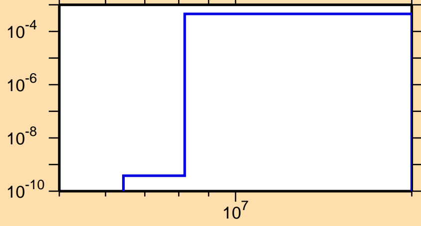
\sigma vs. E for ^{82}\text{Rb}(n,p\alpha)
