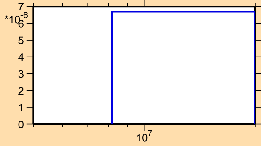
\sigma vs. E for ^{82}\text{Rb}(n,nd)
