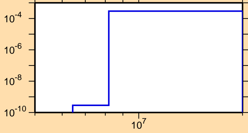
\sigma vs. E for ^{82}\text{Rb}(n,t)
