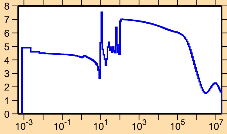
\sigma vs. E for ^{82}\text{Rb}(n,\text{el.})
