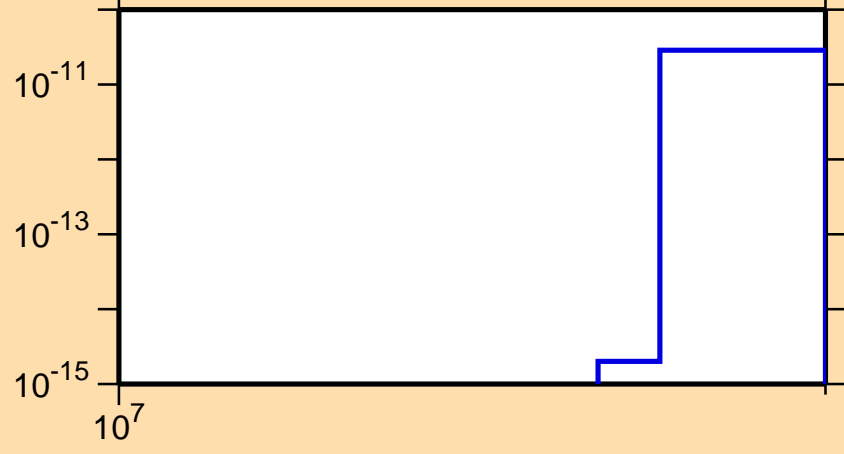
\sigma vs. E for ^{82}\text{Rb} (mt 45)
