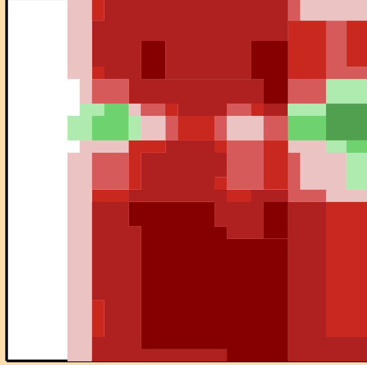
\Delta\sigma/\sigma vs. E for ^{82}\text{Rb}(n,n\text{cont.})
