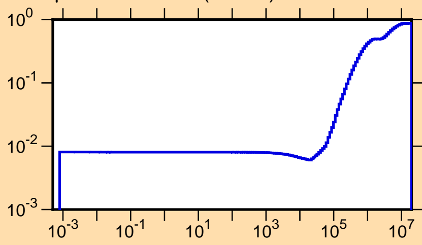
\mu vs. E for ^{83}\text{Rb}(\text{mt251})
