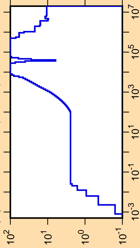
\Delta\mu/\mu vs. E for ^{83}\text{Rb}(\text{mt251})
