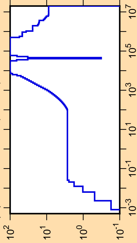
\Delta\mu/\mu vs. E for ^{84}\text{Rb}(\text{mt251})
