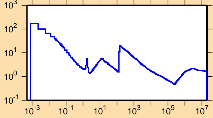
\sigma vs. E for ^{84}\text{Rb}(n,\text{nonel.})
