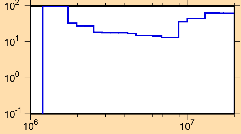
\Delta\sigma/\sigma vs. E for ^{84}\text{Rb}(n,n\text{cont.})
