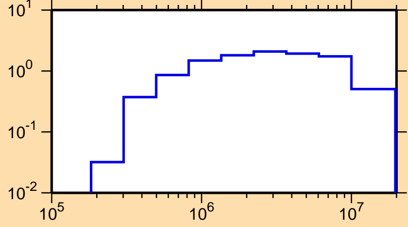
\sigma vs. E for ^{84}\text{Rb}(n,\text{inel.})
