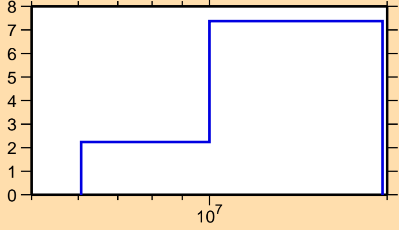
\Delta\sigma/\sigma vs. E for ^{84}\text{Rb}(n,\text{tot.})
