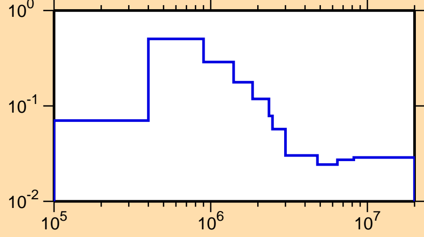
\sigma vs. E for ^{84}\text{Rb}(n,n_1)
