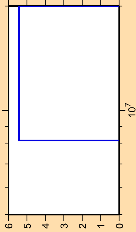
\Delta\sigma/\sigma vs. E for ^{84}\text{Rb}(n,nt)
