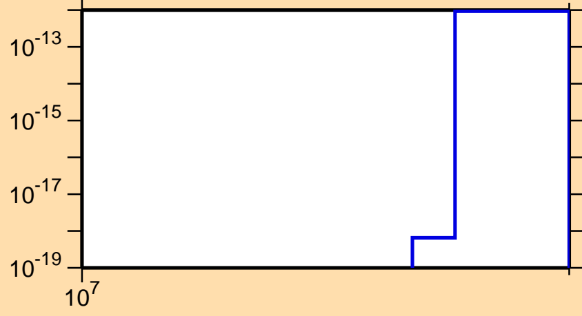
\sigma vs. E for ^{84}\text{Rb}(n,pd)
