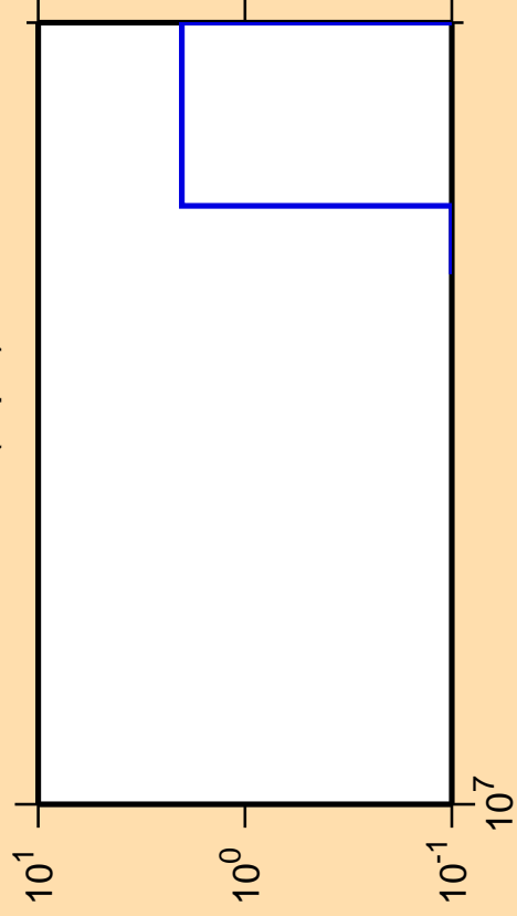
\Delta\sigma/\sigma vs. E for ^{84}\text{Rb}(n,pd)
