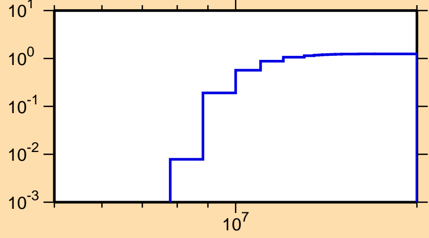
\sigma vs. E for ^{84}\text{Rb}(n,2n)
