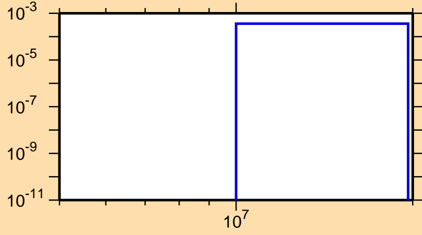
\sigma vs. E for ^{84}\text{Rb}(n,n\alpha)
