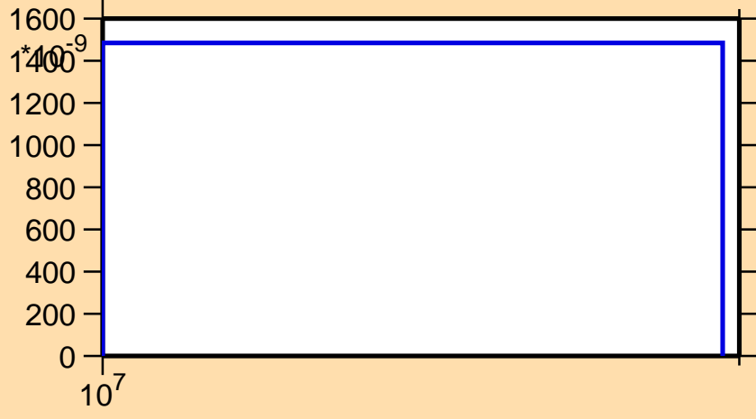
\sigma vs. E for ^{84}\text{Rb}(n,nd)
