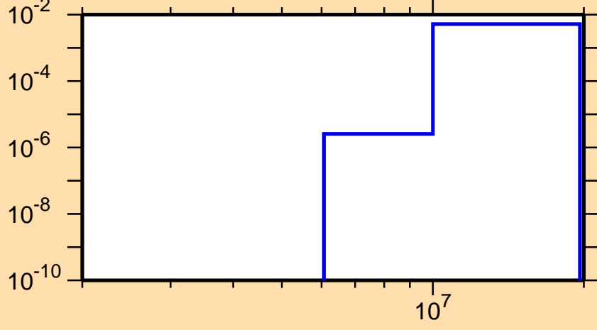
\sigma vs. E for ^{84}\text{Rb}(n,d)
