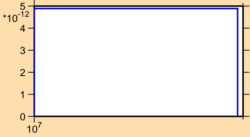
\sigma vs. E for ^{84}\text{Rb}(n,2n\alpha)
