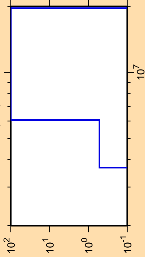
\Delta\sigma/\sigma vs. E for ^{84}\text{Rb}(n,d)
