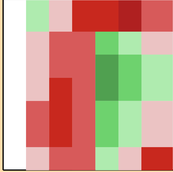
\Delta\sigma/\sigma vs. E for ^{84}\text{Rb}(n,n\text{cont.})
