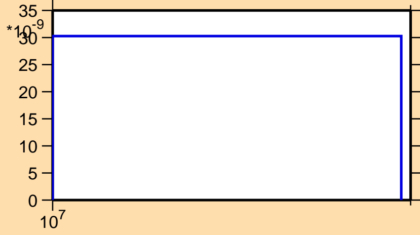
\sigma vs. E for ^{84}\text{Rb}(n,\text{He}3)
