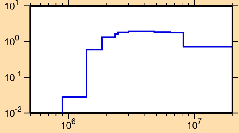
\sigma vs. E for ^{84}\text{Rb}(n,n\text{cont.})
