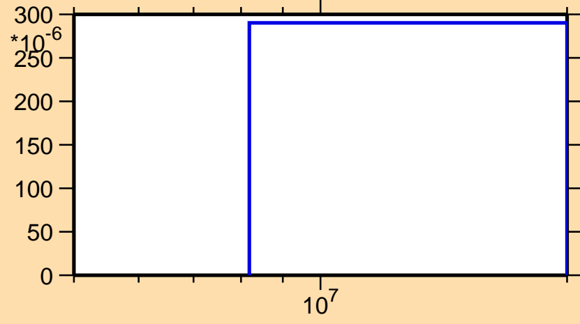
\sigma vs. E for ^{84}\text{Rb}(n,\alpha)
