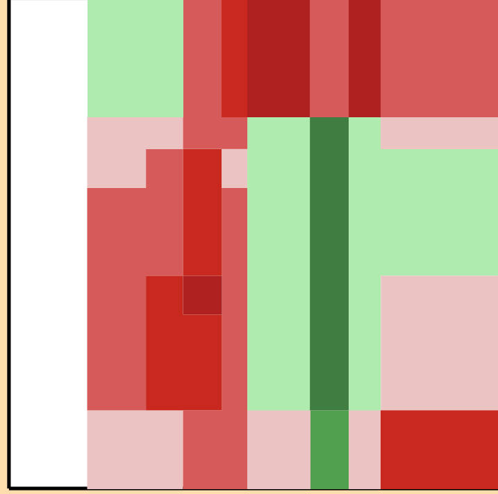
\Delta\sigma/\sigma vs. E for ^{84}\text{Rb}(n,ncont.)
