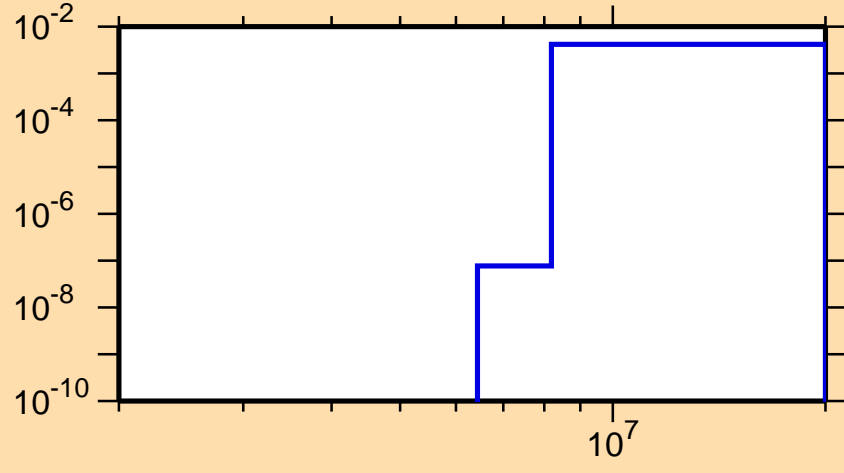
\sigma vs. E for ^{84}\text{Rb}(n,d)
