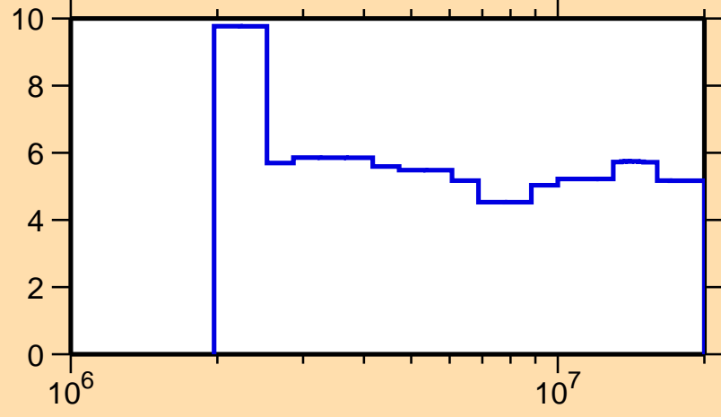
\Delta\sigma/\sigma vs. E for ^{85}\text{Rb}(n,n\text{onel.})
