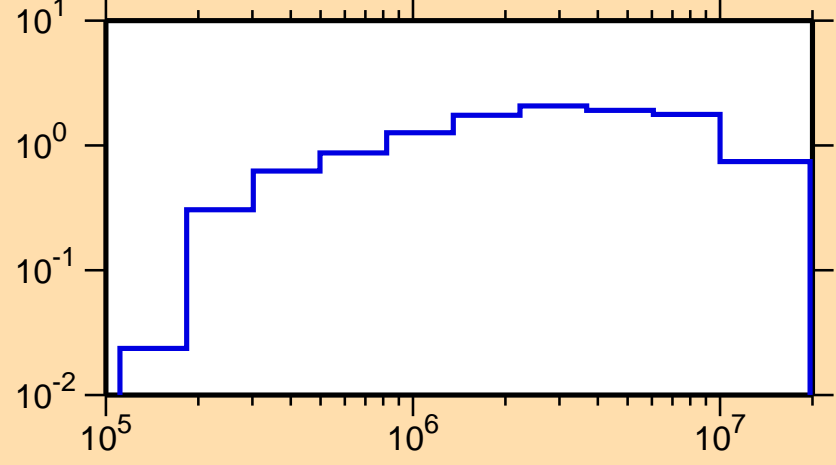
\sigma vs. E for ^{85}\text{Rb}(n,\text{inel.})
