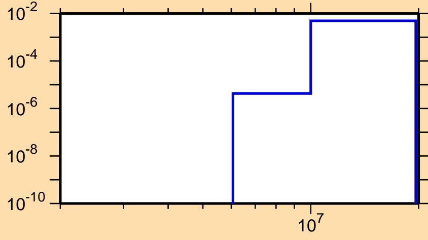
\sigma vs. E for ^{85}\text{Rb}(n,d)
