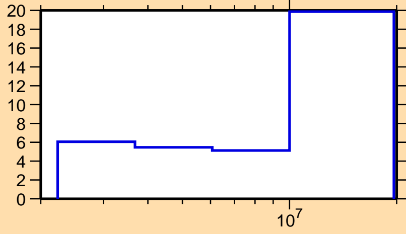
\Delta\sigma/\sigma vs. E for ^{85}\text{Rb}(n,n\text{cont.})
