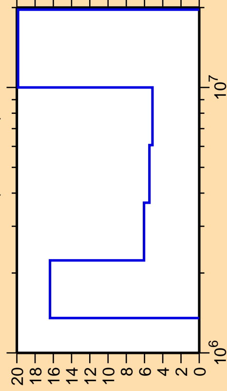
\Delta\sigma/\sigma vs. E for ^{85}\text{Rb}(n,\text{ncont.})
