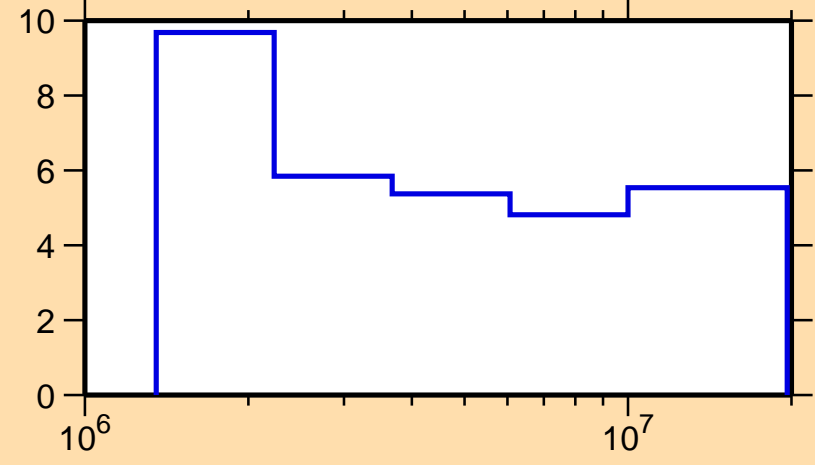
\Delta\sigma/\sigma vs. E for ^{85}\text{Rb}(n,n\text{nonel.})
