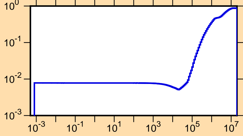
\mu vs. E for ^{86}\text{Rb}(\text{mt251})
