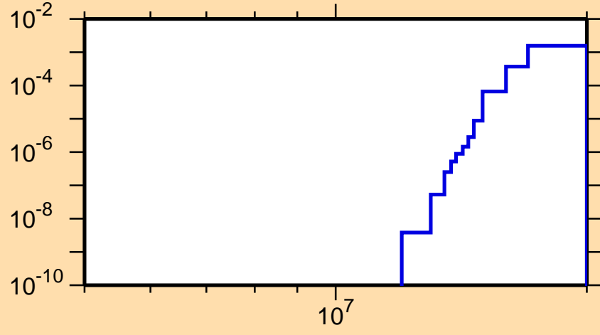
\sigma vs. E for ^{86}\text{Rb}(n,\alpha)
