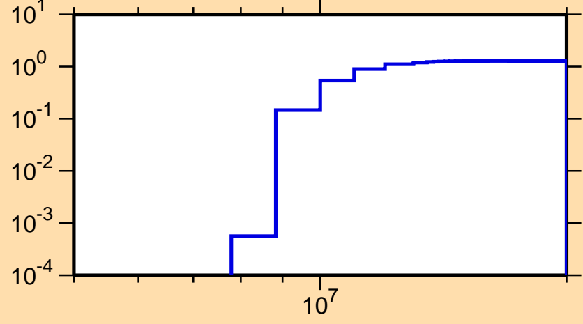
\sigma vs. E for ^{86}\text{Rb}(n,2n)
