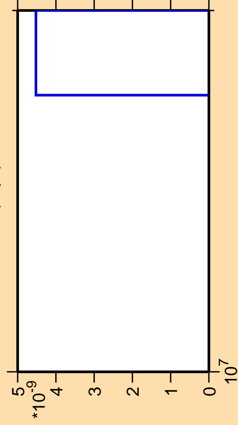
\Delta\sigma/\sigma vs. E for ^{86}\text{Rb}(n,\text{pt})
