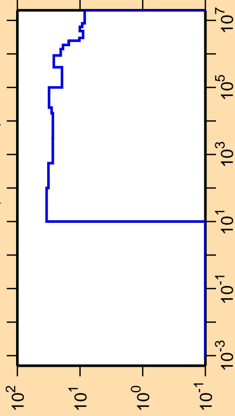
\Delta\sigma/\sigma vs. E for ^{86}\text{Rb}(n,\text{nonel.})
