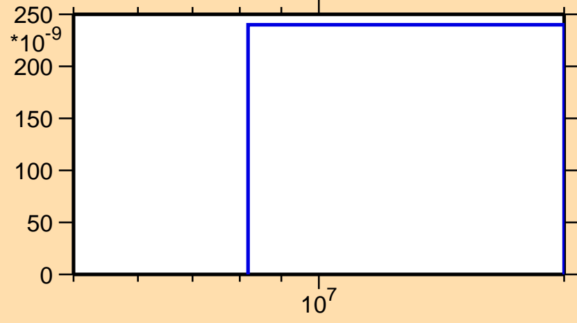
\sigma vs. E for ^{86}\text{Rb}(n,2np)
