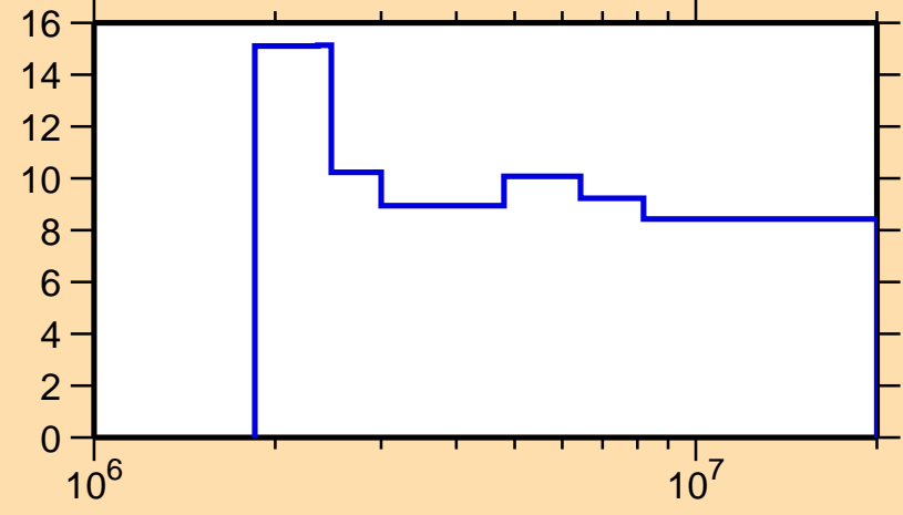
\Delta\sigma/\sigma vs. E for ^{86}\text{Rb}(n,n\text{onel.})
