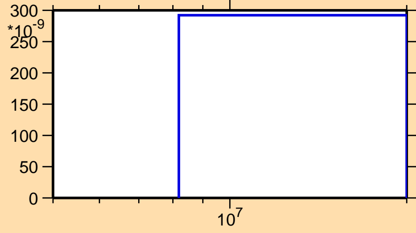
\sigma vs. E for ^{86}\text{Rb}(n,\text{nd})
