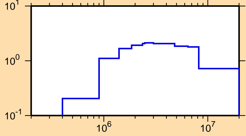
\sigma vs. E for ^{86}\text{Rb}(n,\text{inel.})
